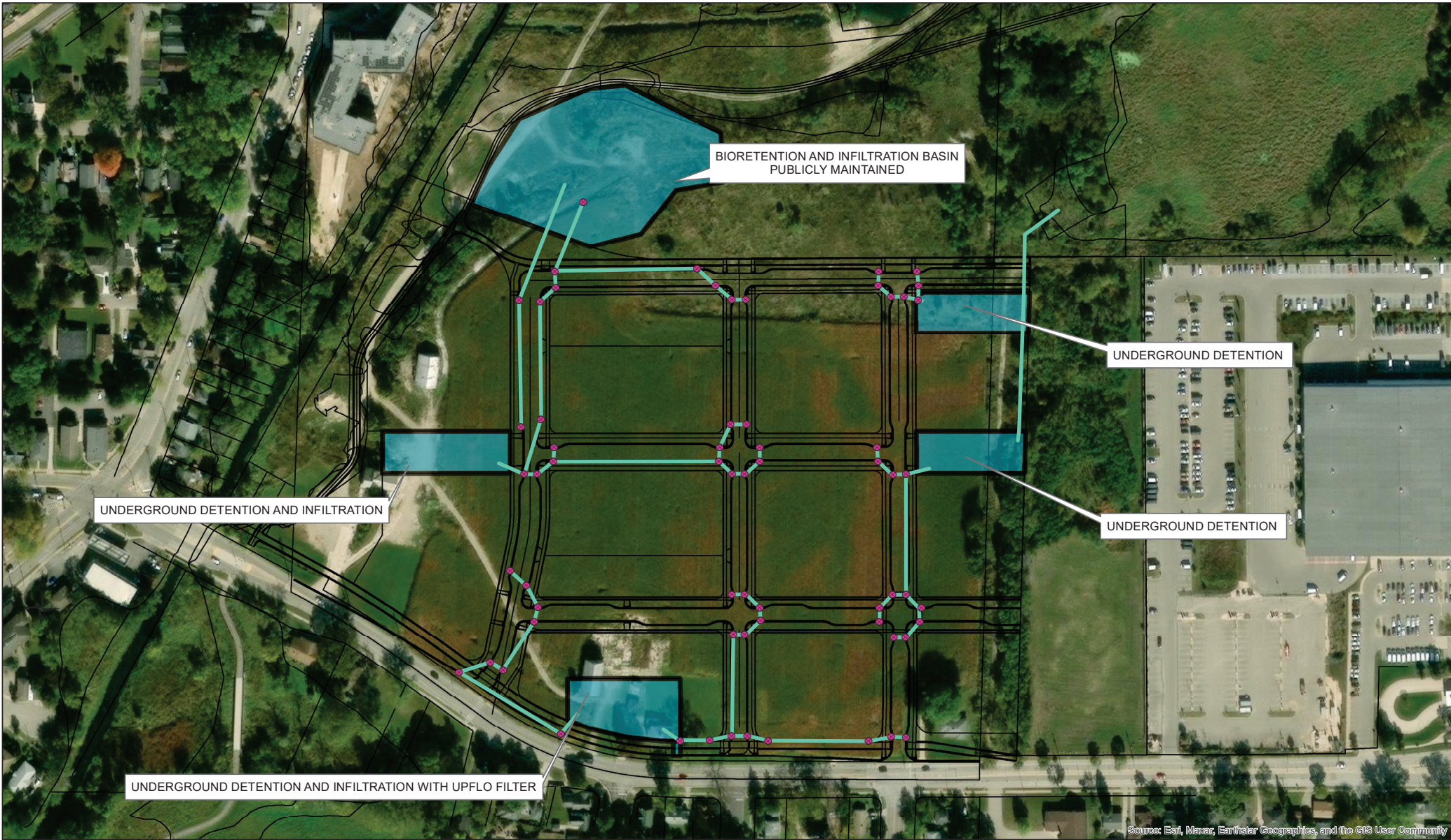
Starkweather Storm Sewer Layout and Treatment Areas 6/26/2025 M:\PlanVault\PlatDrainagePlans\Voit_StarkweatherPlat_2024\Storm Layout and Sizing
