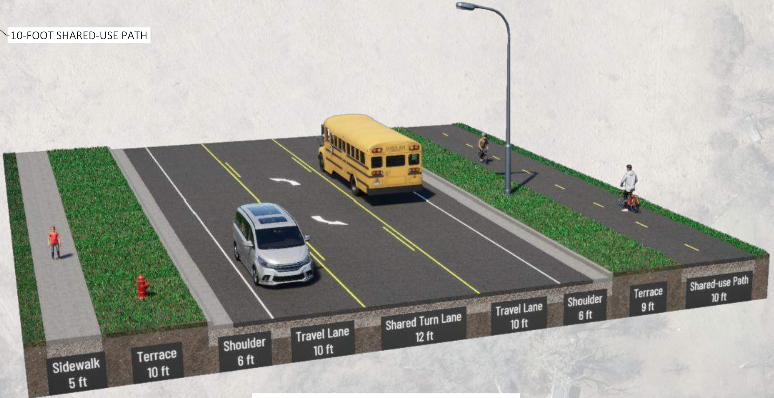
S HIGH POINT RD TYPICAL SECTION TWO-WAY LEFT-TURN LANE
