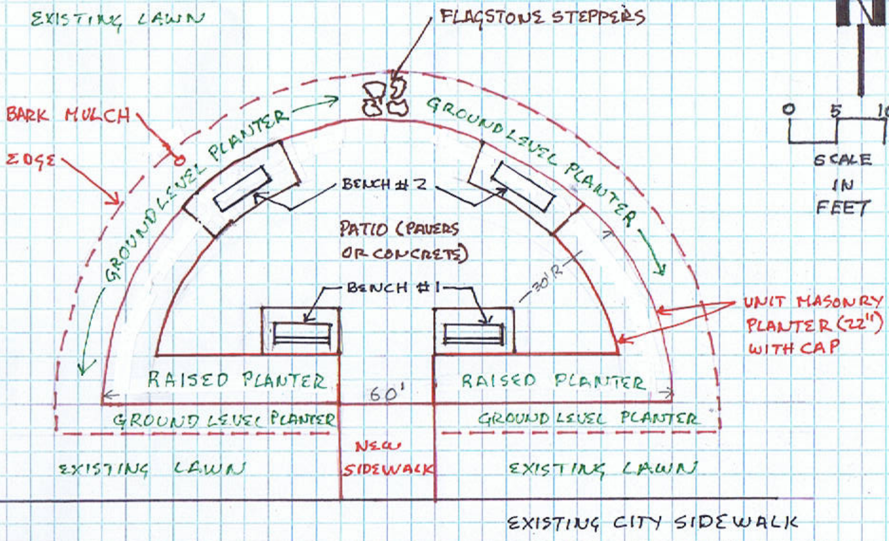
PROPOSED LAYOUT PLAN - 1" = 10'
