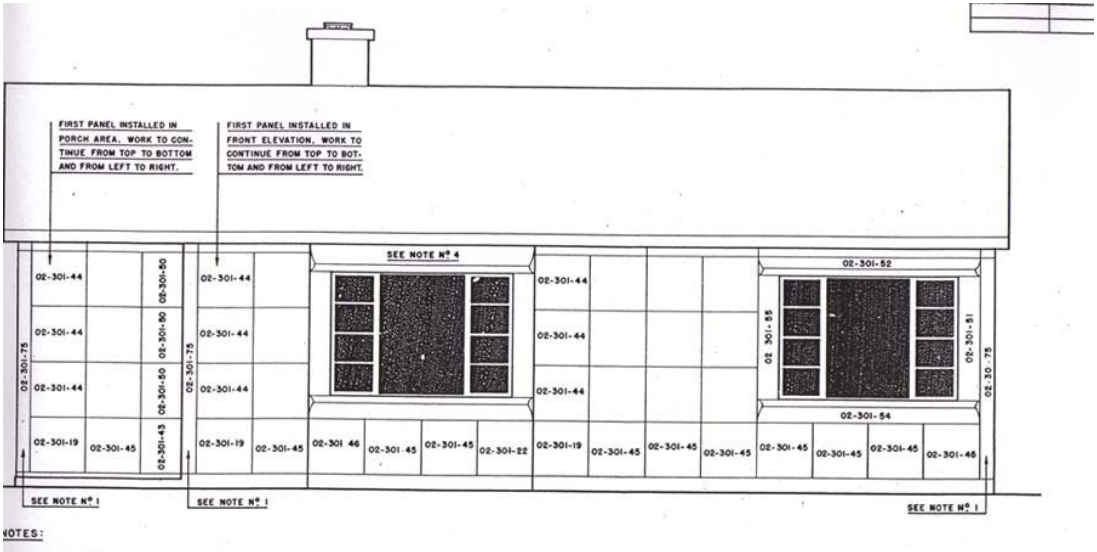
FRONT ELEVATION - From Factory Erection Manual
