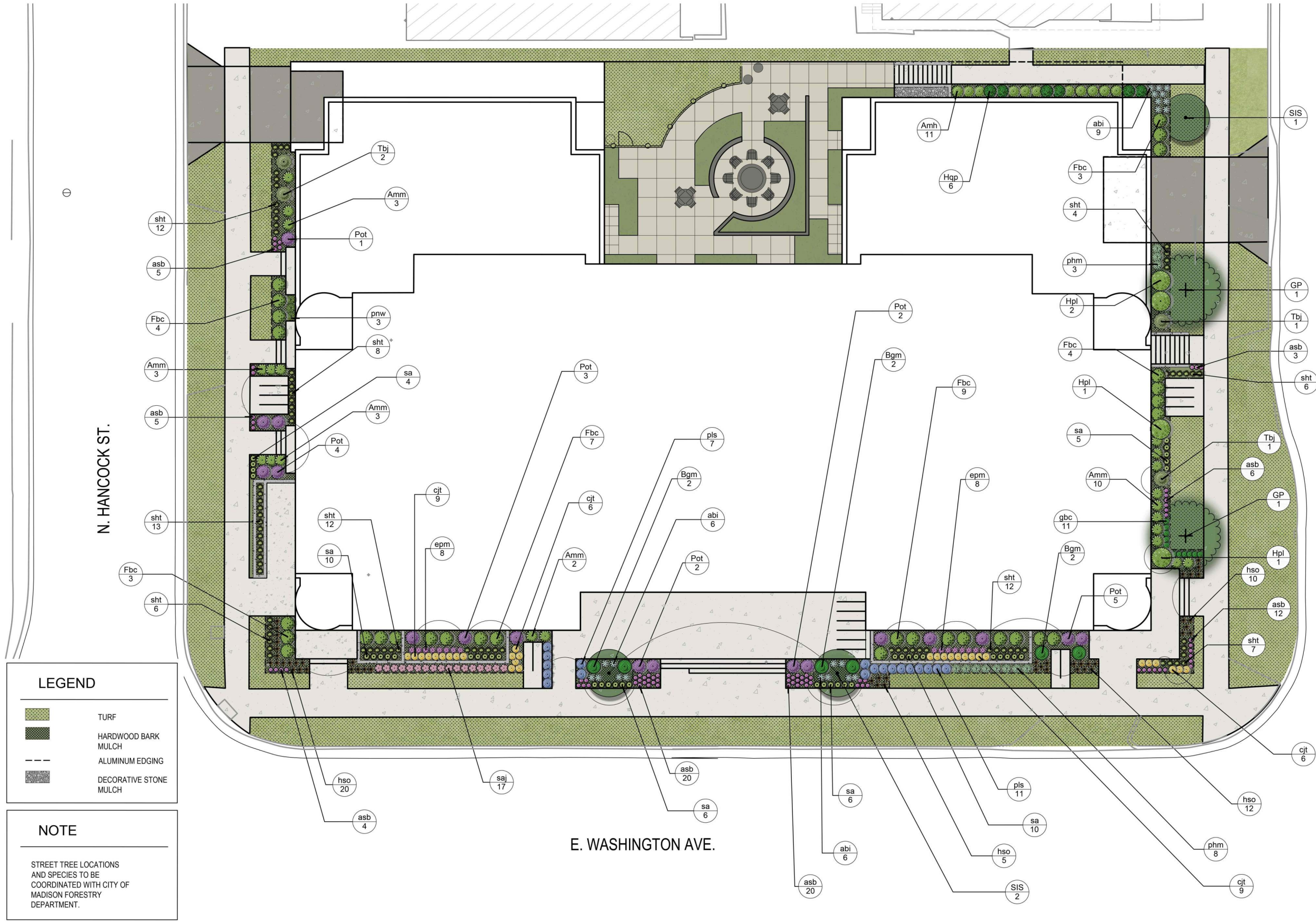
1 Landscape Plan SCALE: 1" = 10'-0"
