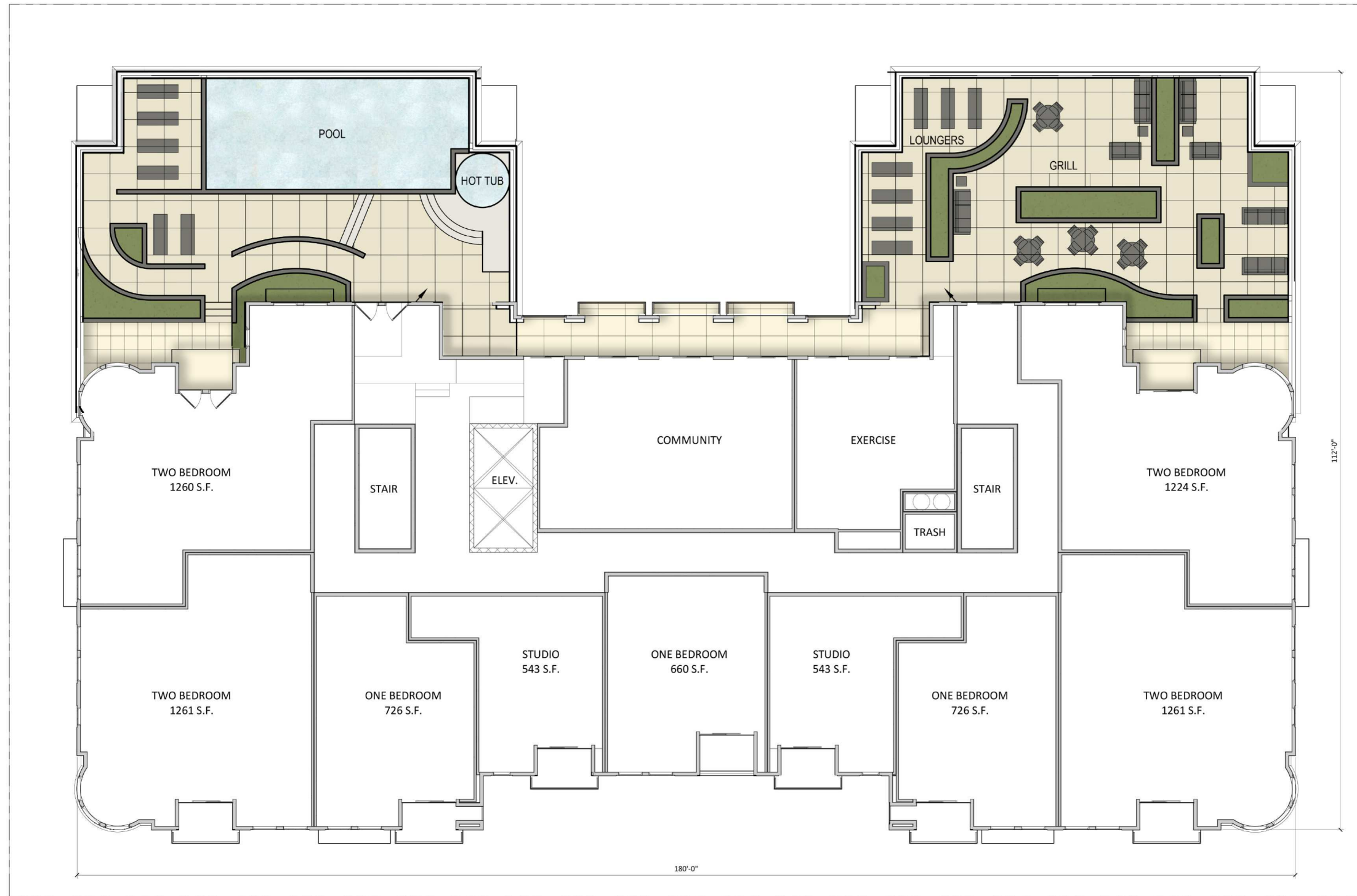
1 SEVENTH FLOOR PLAN A-1.7 1/8" = 1'-0"
