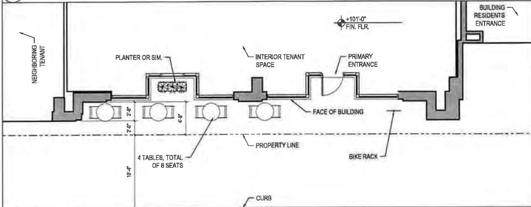
1 OVERALL BUILDING LAYOUT 1"=20'
