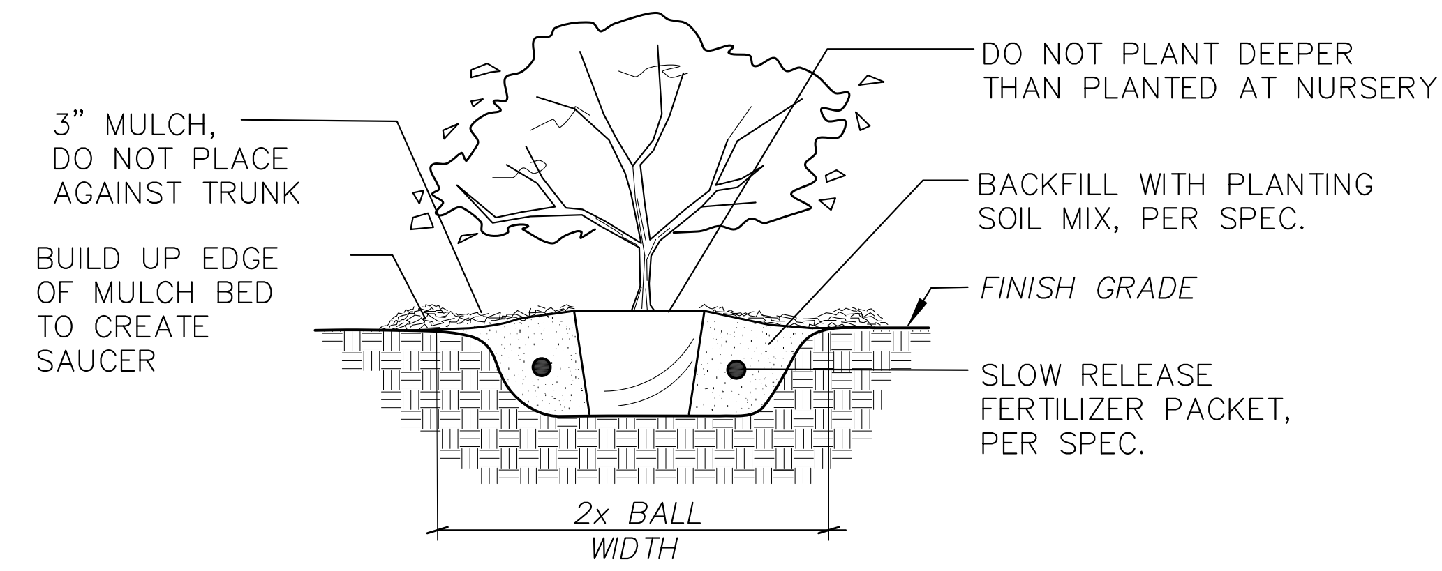
3 CONTAINER PLANTING DETAIL L102 NTS
