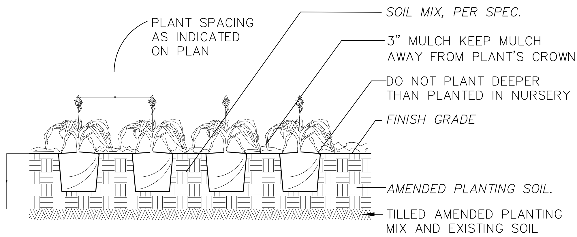
5 GROUNDCOVER / PERENNIAL PLANTING DETAIL L102 NTS
