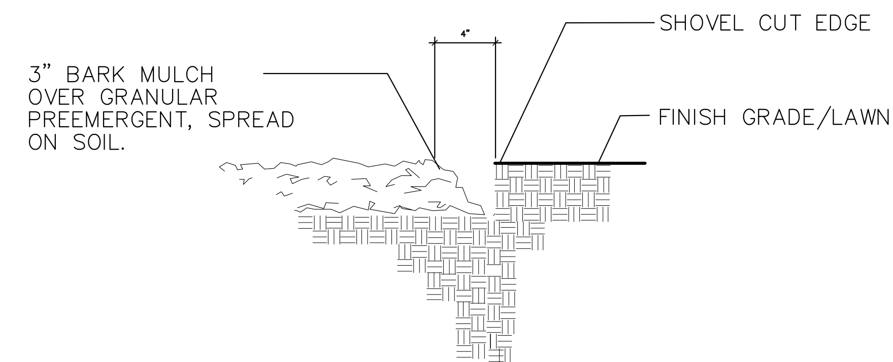
7 BARK MULCH/SHOVEL CUT EDGE DETAIL L102 NTS
