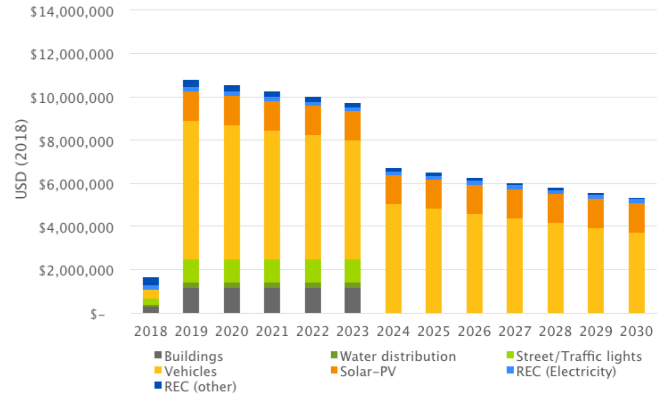
FIGURE 2 15. ANNUAL INVESTMENTS IN SCENARIO 3: 100% RENEWABLE ENERGY AND ZERO NET CARBON BY 2030
