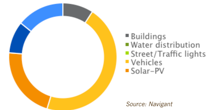
FIGURE 2-4. CUMULATIVE INVESTMENTS IN SCENARIO 1: 100% RENEWABLE ENERGY AND ZERO NET CARBON BY 2020
