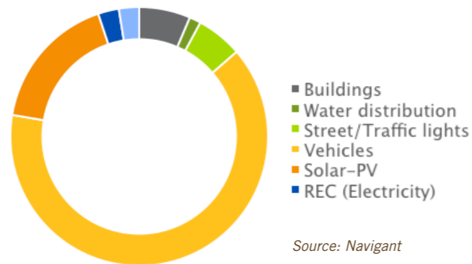
FIGURE 2-16. CUMULATIVE INVESTMENTS IN SCENARIO 3: 100% RENEWABLE ENERGY AND ZERO NET CARBON BY 2030
