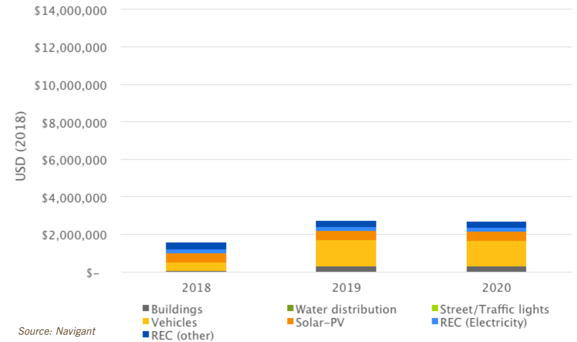
FIGURE 2-3. ANNUAL INVESTMENTS IN SCENARIO 1: 100% RENEWABLE ENERGY AND ZERO NET CARBON BY 2020
