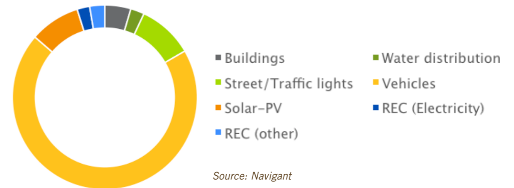
FIGURE 2-10. CUMULATIVE INVESTMENTS IN SCENARIO 2: 100% RENEWABLE ENERGY AND ZERO NET CARBON BY 2023
