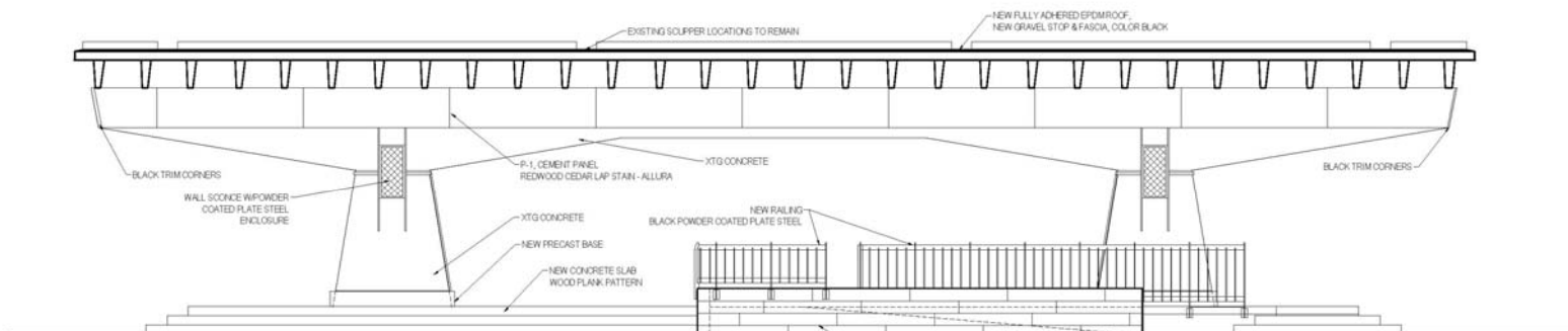
1 SHELTER SOUTH ELEVATION 3/16" = 1'-0"
