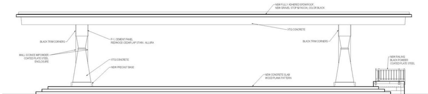
2 SHELTER WEST ELEVATION 3/16" = 1'-0"
