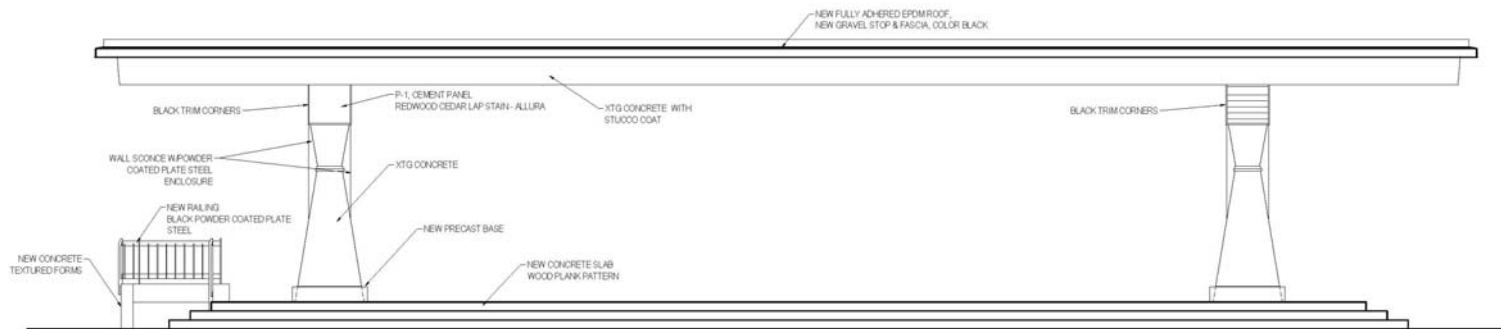
2 SHELTER EAST ELEVATION 3/16" = 1'-0"
