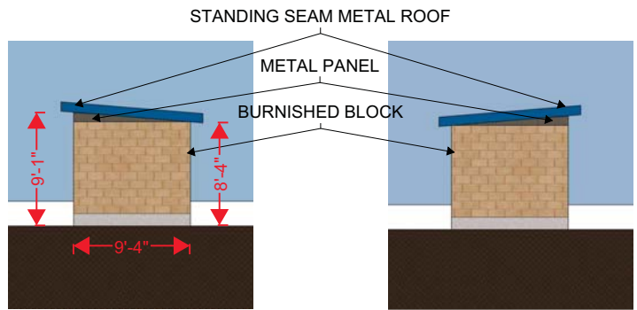
VISITOR DUGOUT - SOUTH ELEVATION
