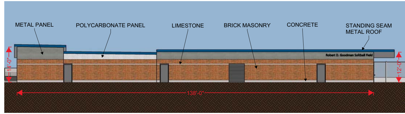
SOFTBALL BUILDING - NORTH ELEVATION WITHOUT FENCE
