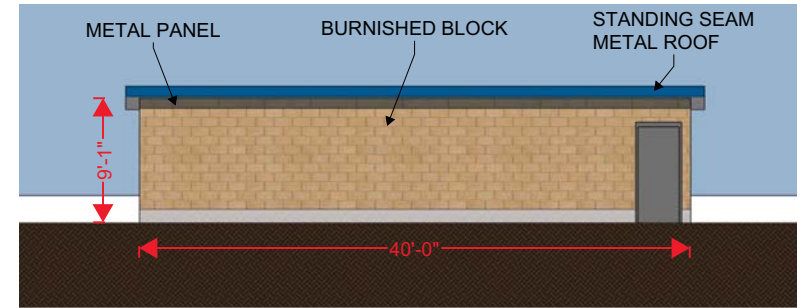
VISITOR DUGOUT - EAST ELEVATION
