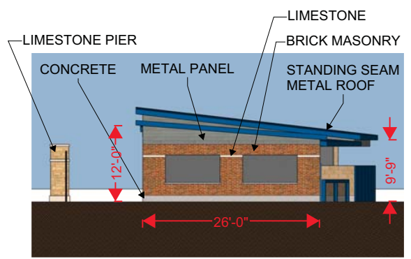
SOFTBALL BUILDING - WEST ELEVATION
