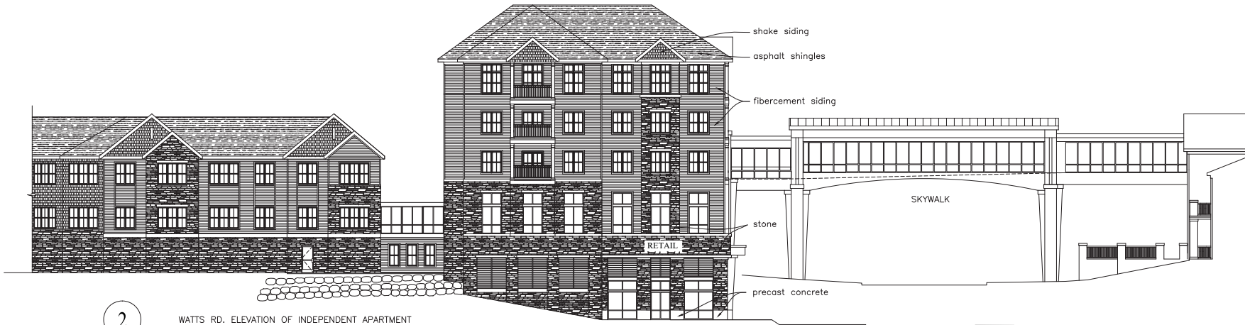
WATTS RD. ELEVATION OF INDEPENDENT APARTMENT
