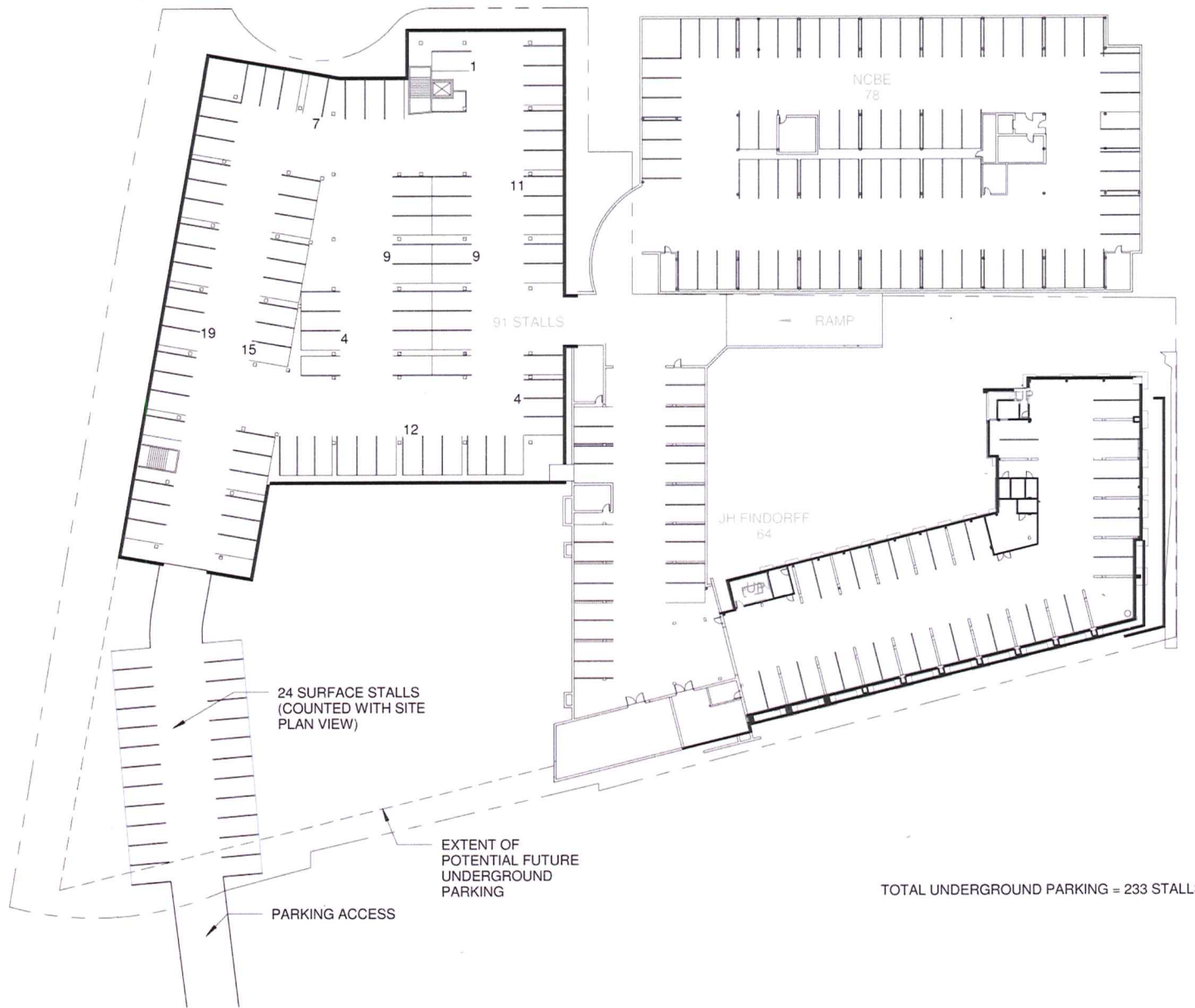
Lower Level Parking Plan
