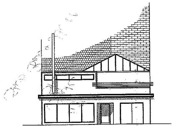
FUTURE CARROLL STREET ELEVATION SCALE: 1/8" = 1'-0"
