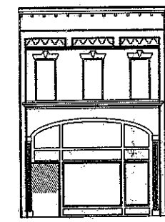
STATE STREET ELEVATION SCALE: 1/8" = 1'-0"
