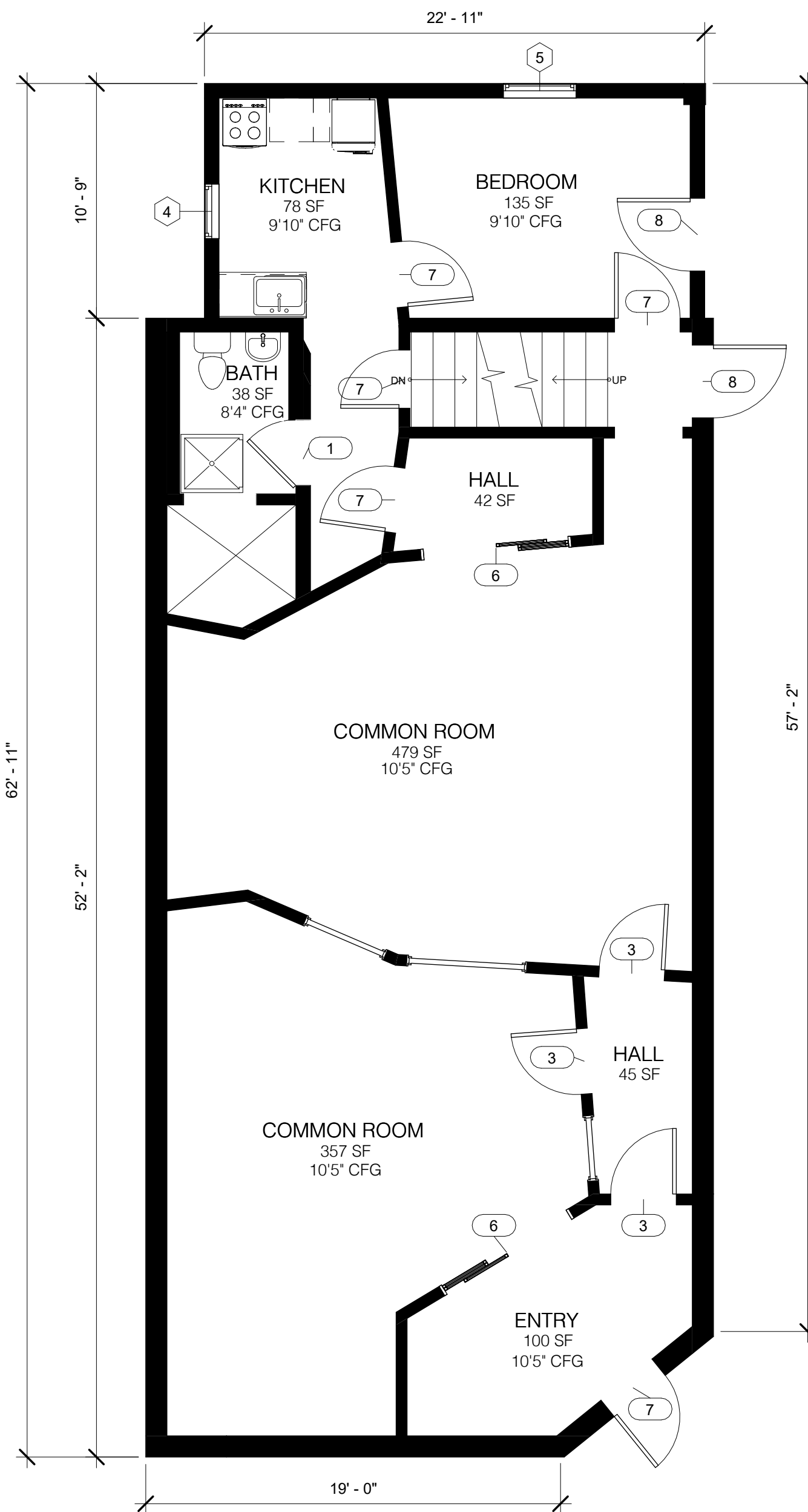
② 1st FLOOR PLAN
