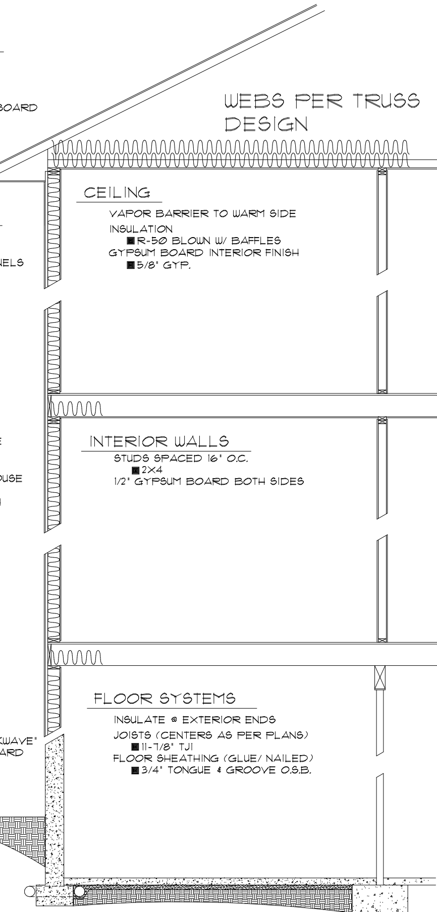
TYPICAL WALL SECTION N.T.S.
