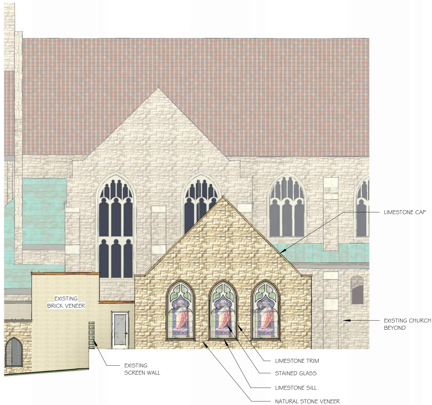
WEST ELEVATION
