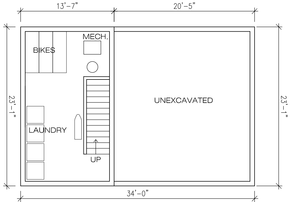
Lower Level Plan - 235 NSF
