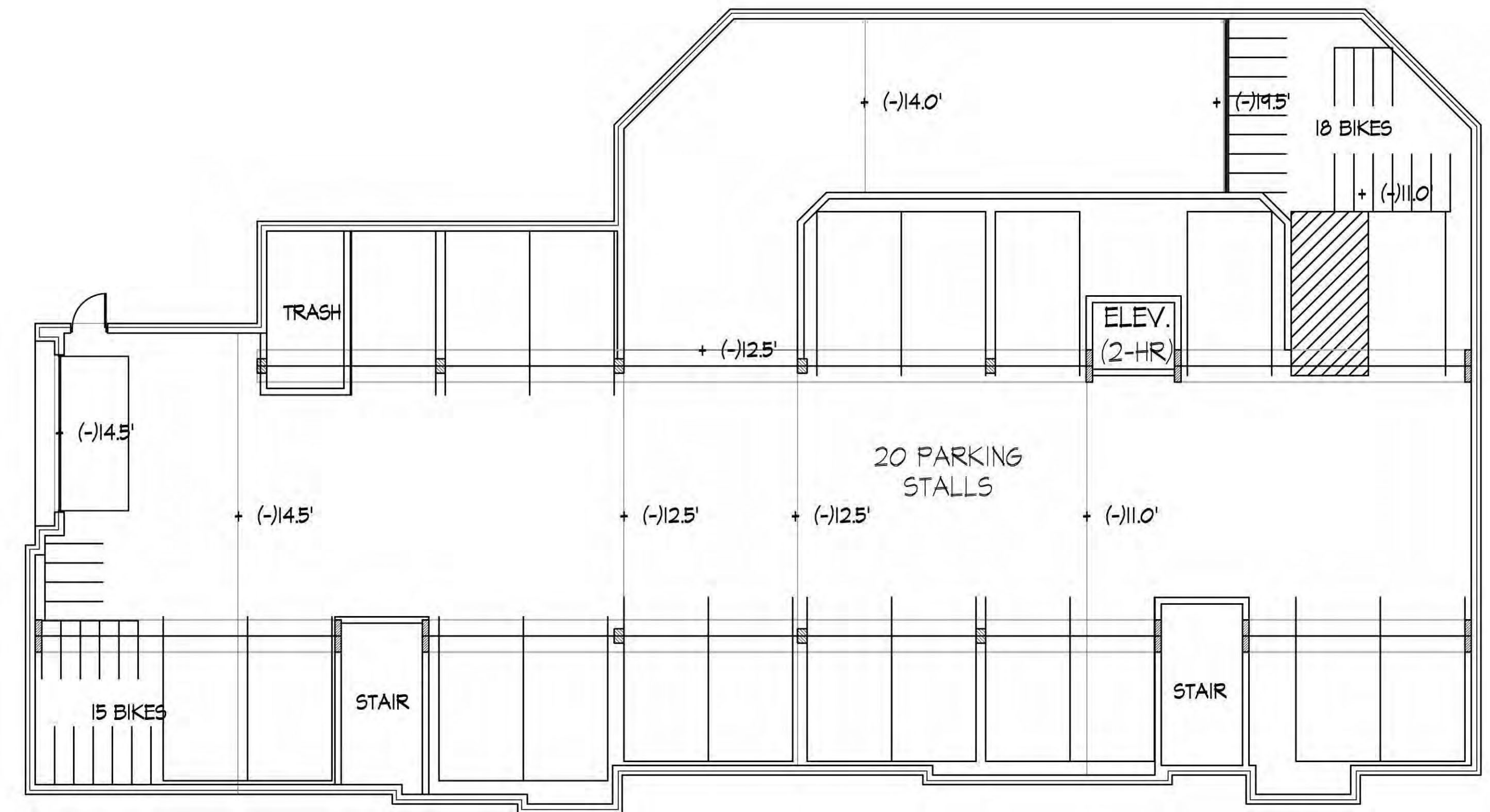
BASEMENT PLAN
