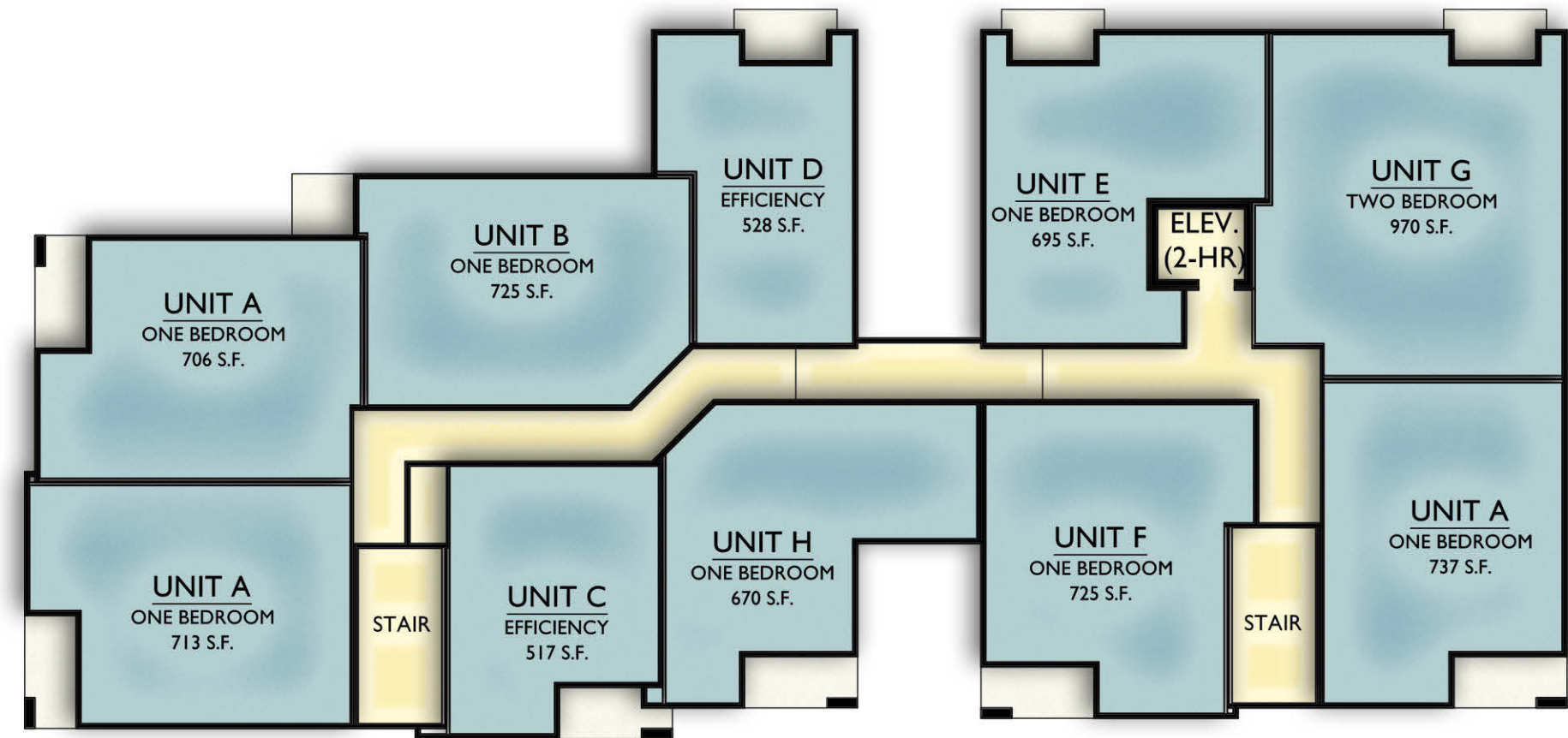
Second - Fourth Floor Plan
