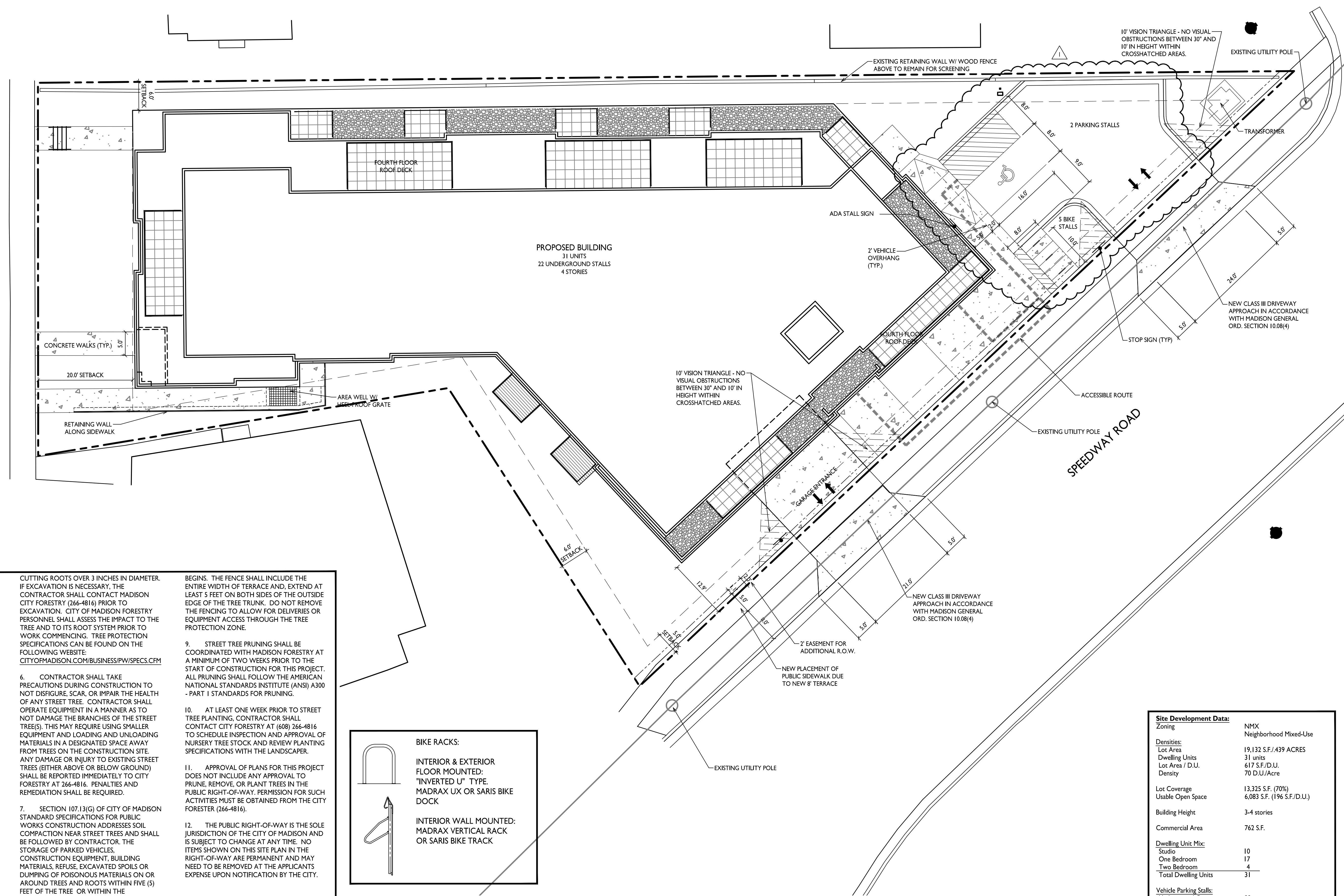
SITE PLAN 1" = 10'-0"
