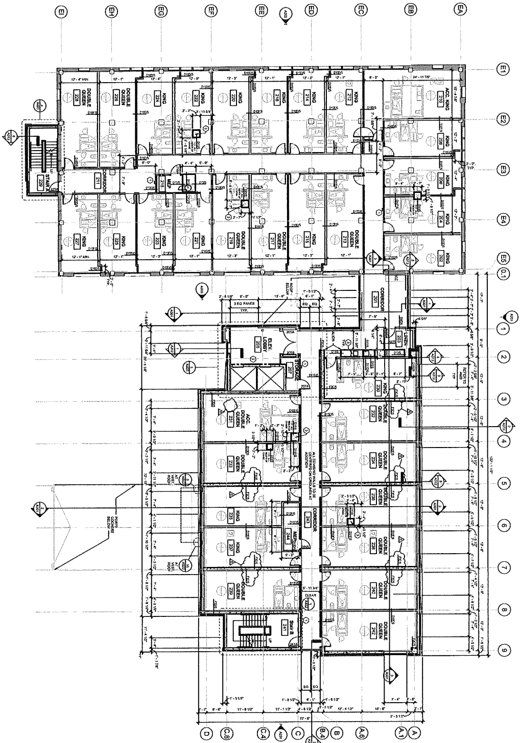
1 SECOND FLOOR PLAN 1/8" = 1'-0"
