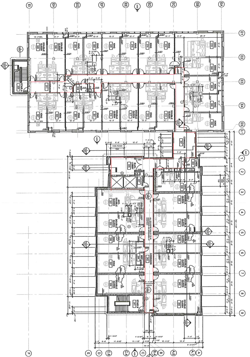
1 THIRD FLOOR PLAN 1/8" = 1'-0"
