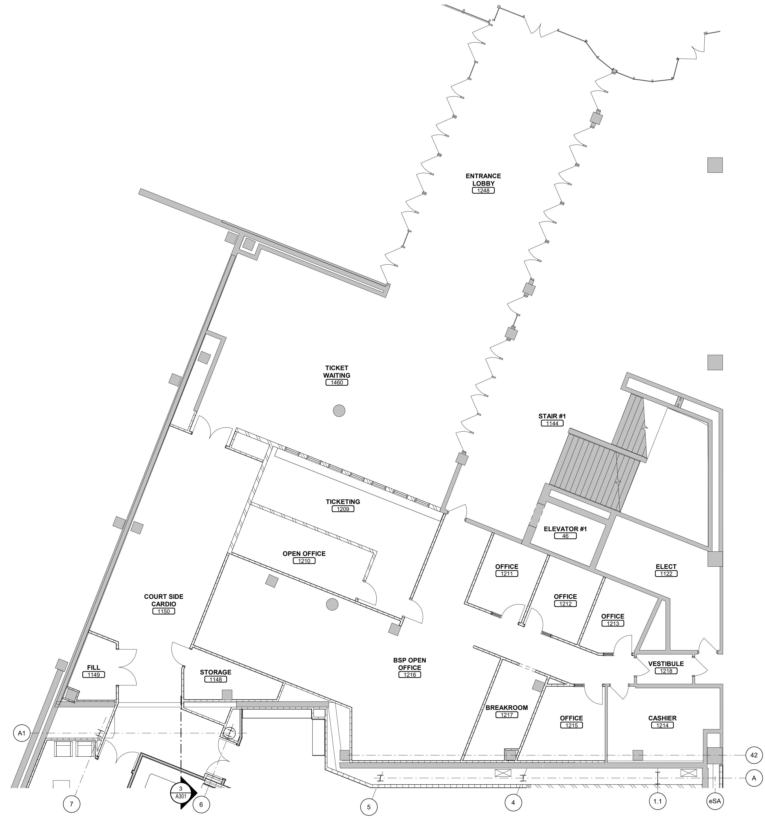
1 A102E AREA F - MAIN CONCOURSE - NEW CONSTRUCTION 1/8" = 1'-0"
