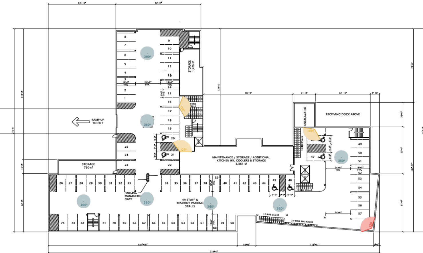
N LOWER LEVEL PLAN 1/16" = 1'-0" @ 24x36
