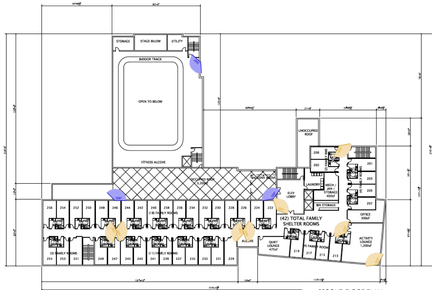
SECOND FLOOR PLAN 1/16" = 1'-0" @ 24x36
