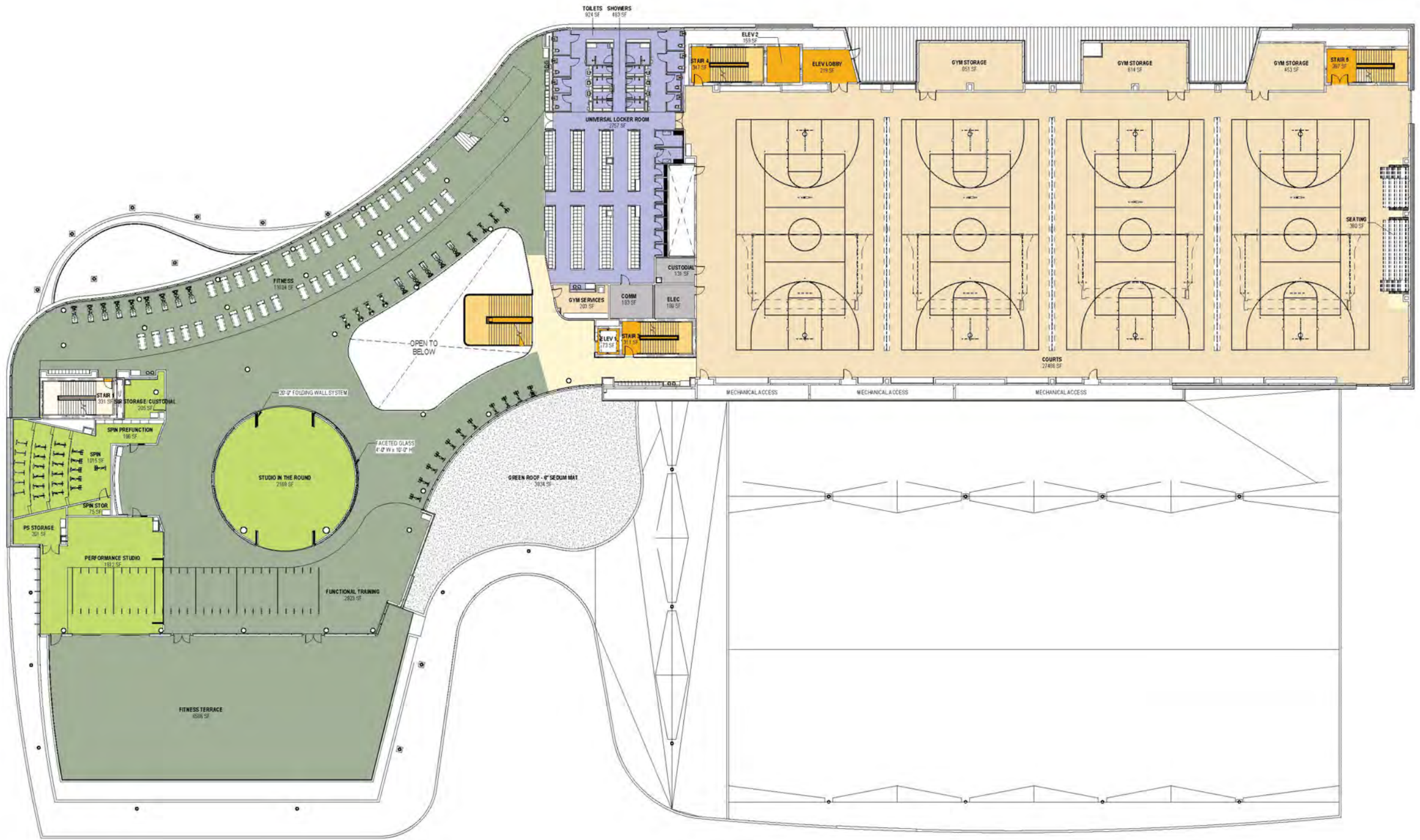
Level 2 Floor Plan
