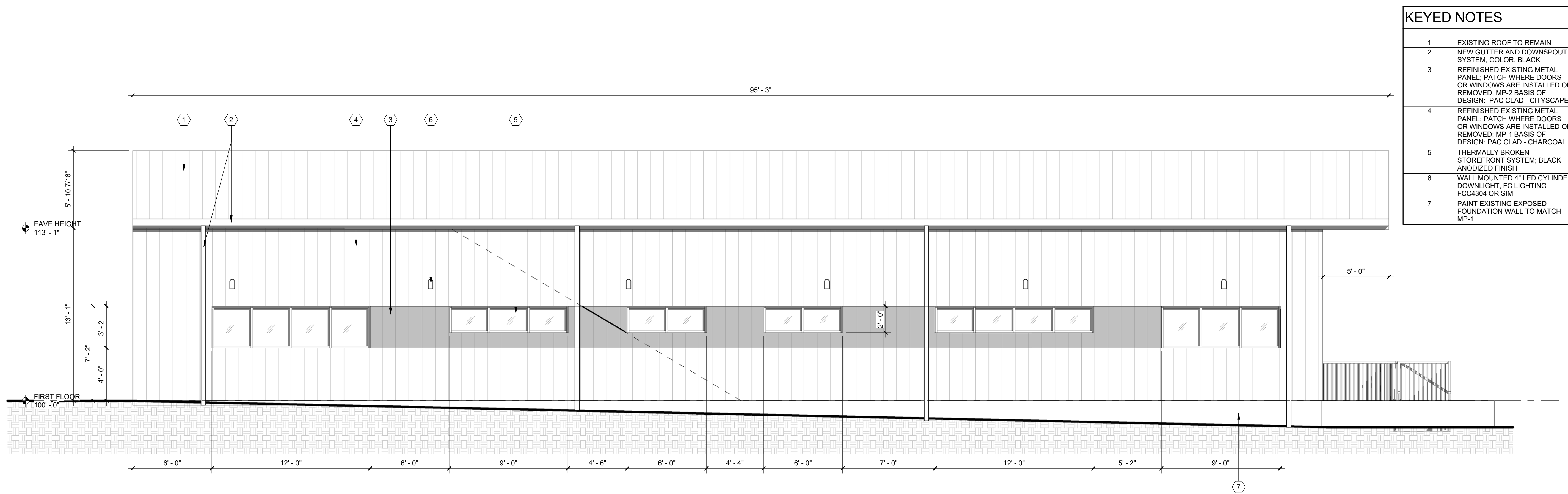
1 NORTH ELEVATION PRESENTATION 1/4" = 1'-0"
