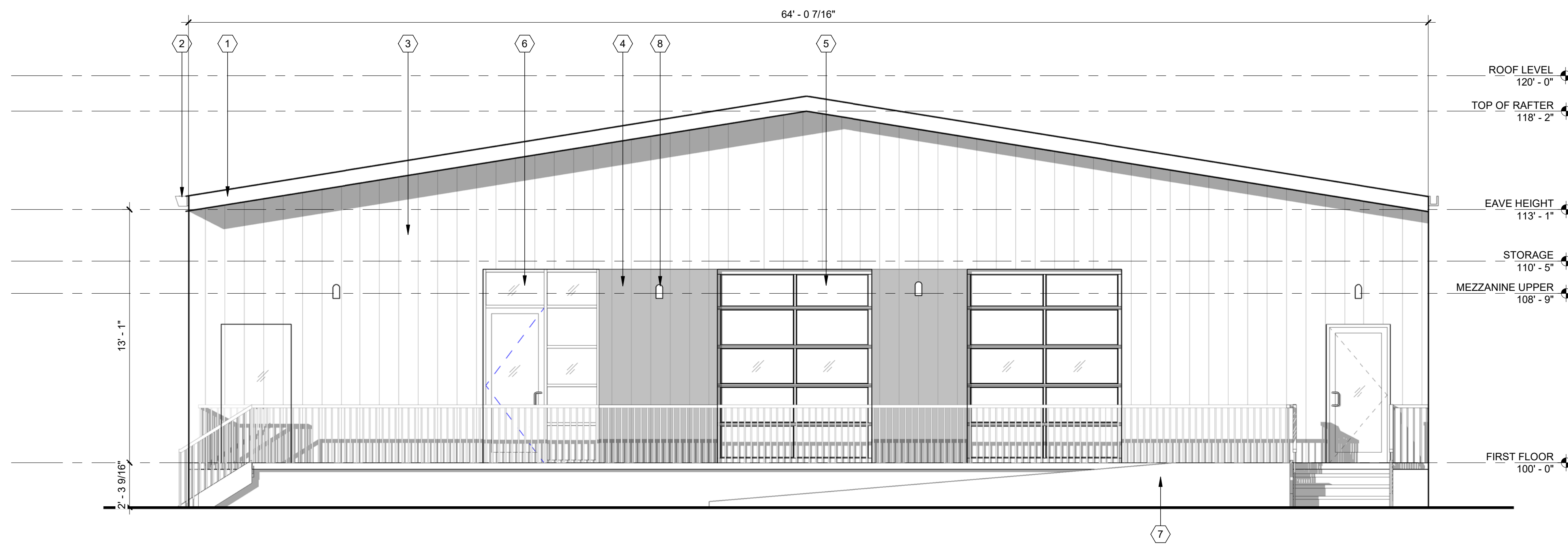
1 WEST ELEVATION FOR CONSTRUCTION 1/4" = 1'-0"
