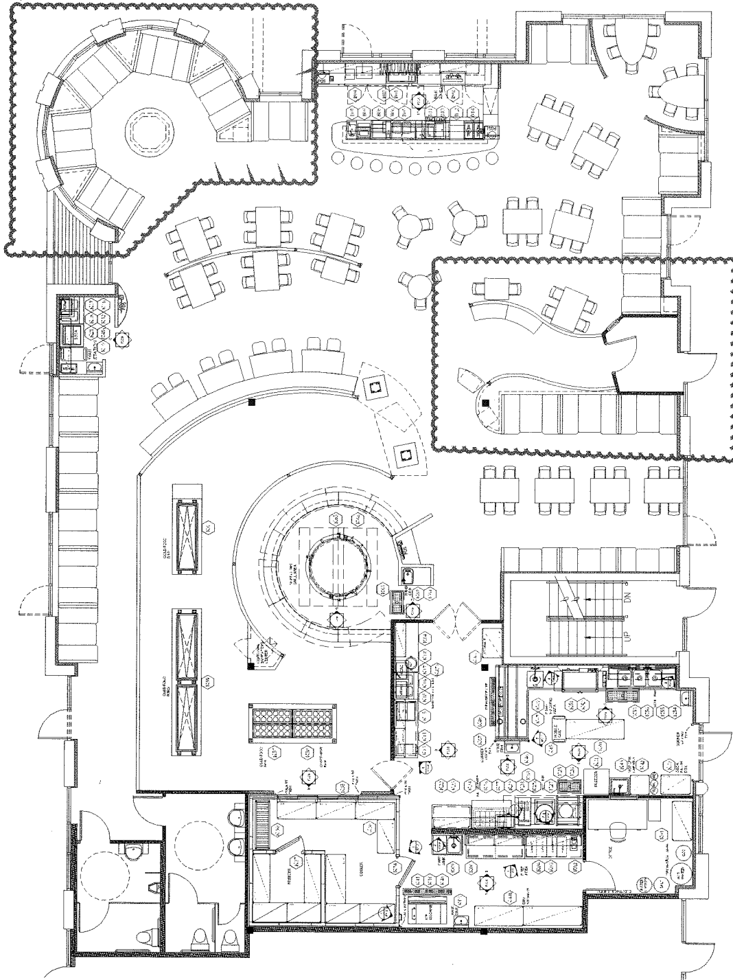
Foodservice Floor Plan Scale: 1/4" = 1'-0"
