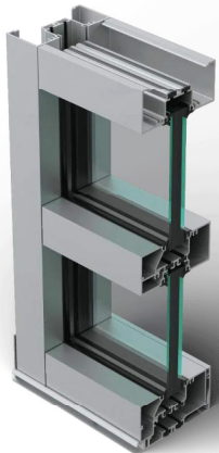
STOREFRONT - KAWNEER 541UT ANODIZED ALUMINUM
