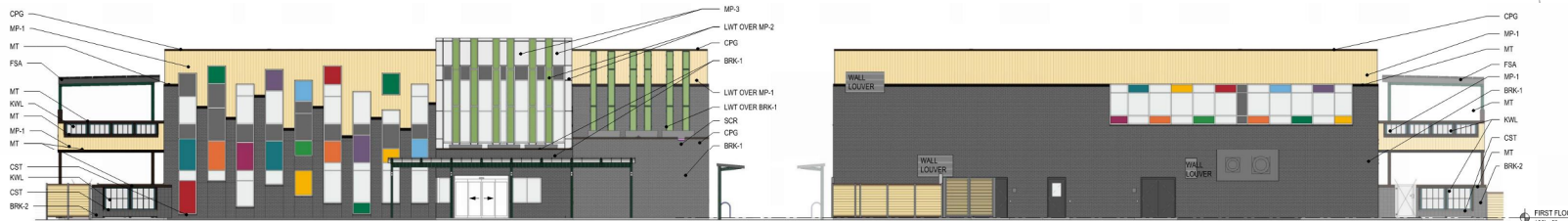
5 SOUTH ELEVATION 332' x 1'-0"
