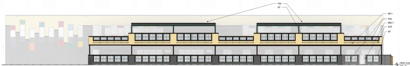
3 EAST ELEVATION 332' x 1'-0"
