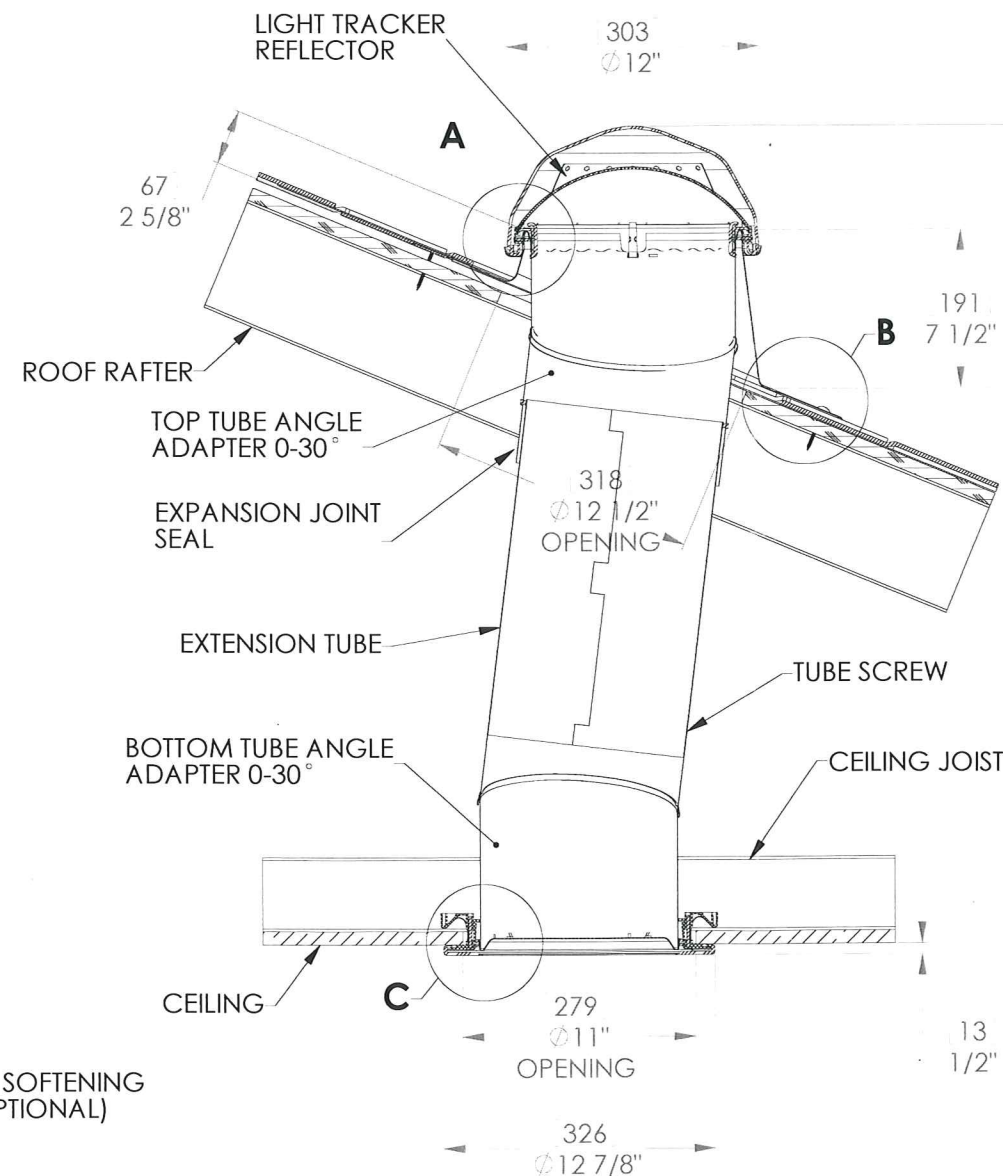
FULL SECTION SCALE 1:1
