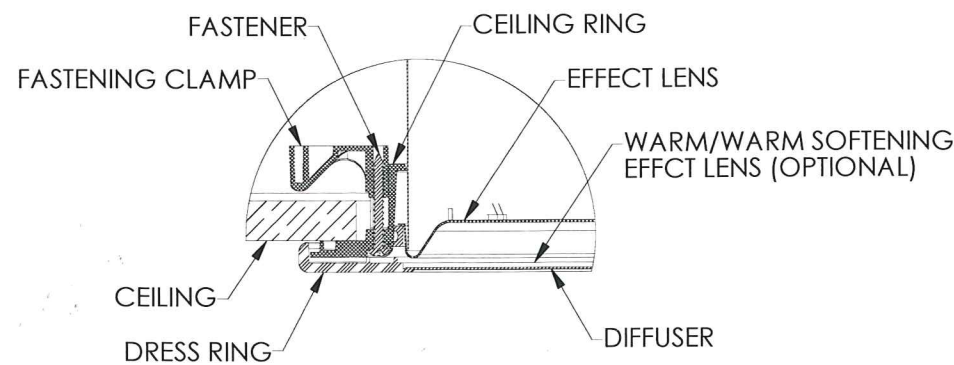
DETAIL C SCALE 3 : 1
