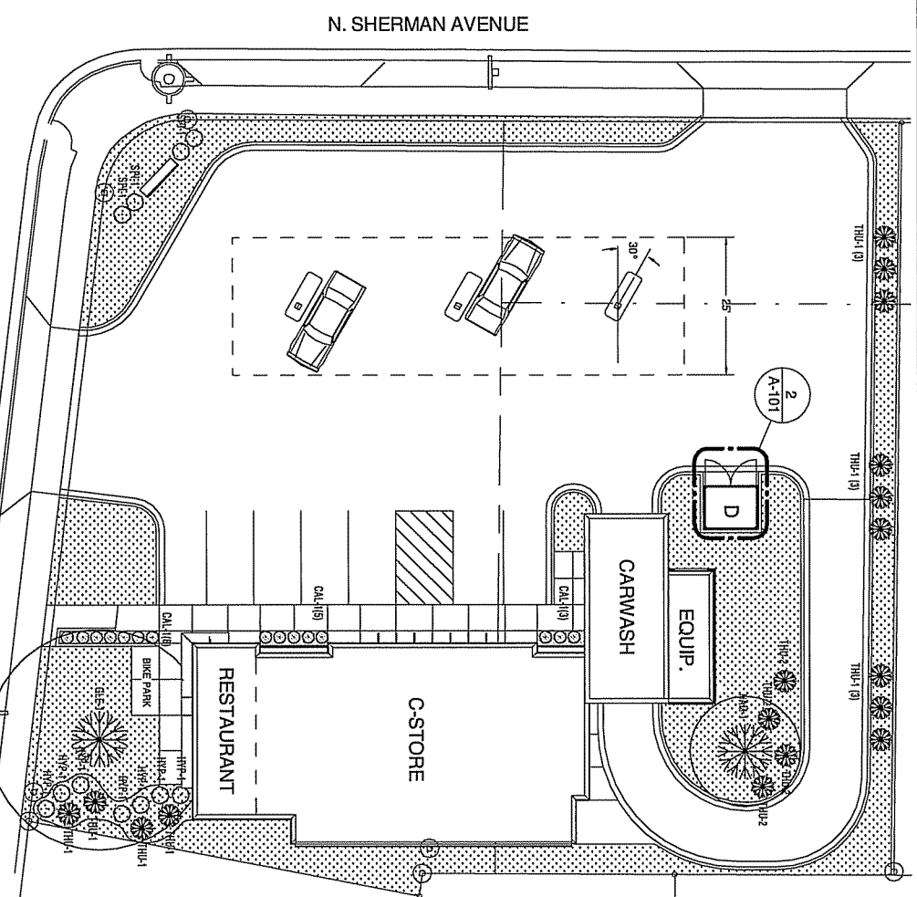
1 LANDSCAPE PLAN 11X17 1" = 20'-0"
