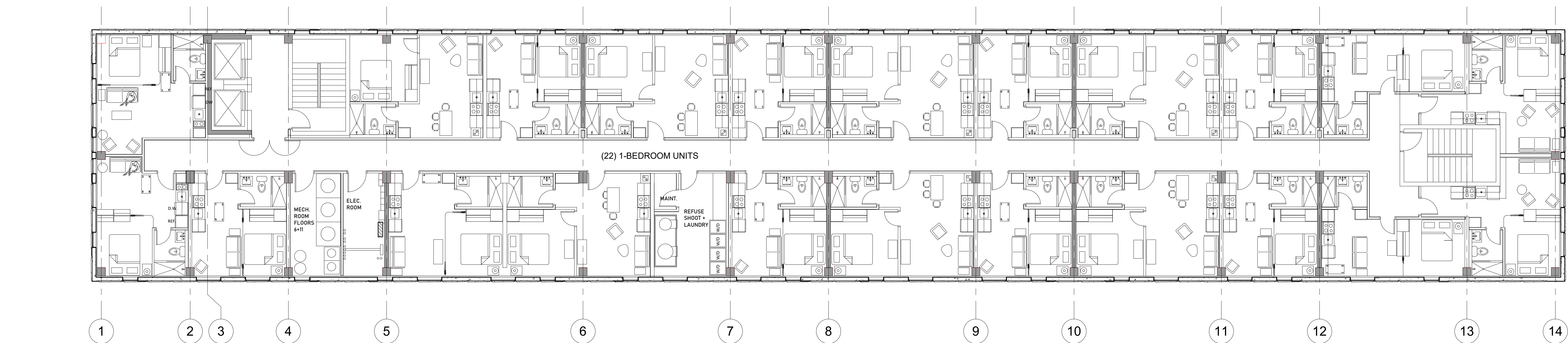
① LEVELS 5, 6 AND 11 1/8" = 1'-0"
