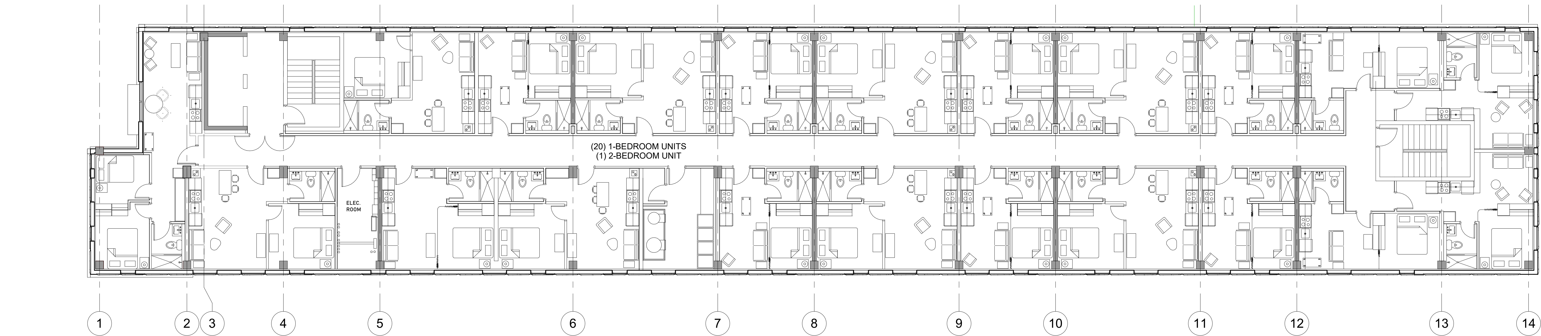
② LEVELS 3 & 4 1/8" = 1'-0"
