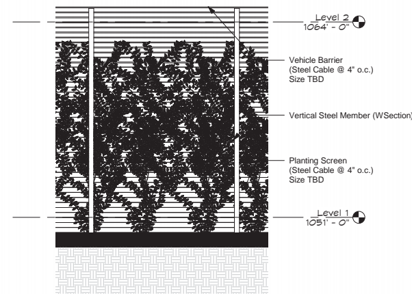
3 TYPICAL PARKING SCREEN A202c 1/4" = 1'-0"
