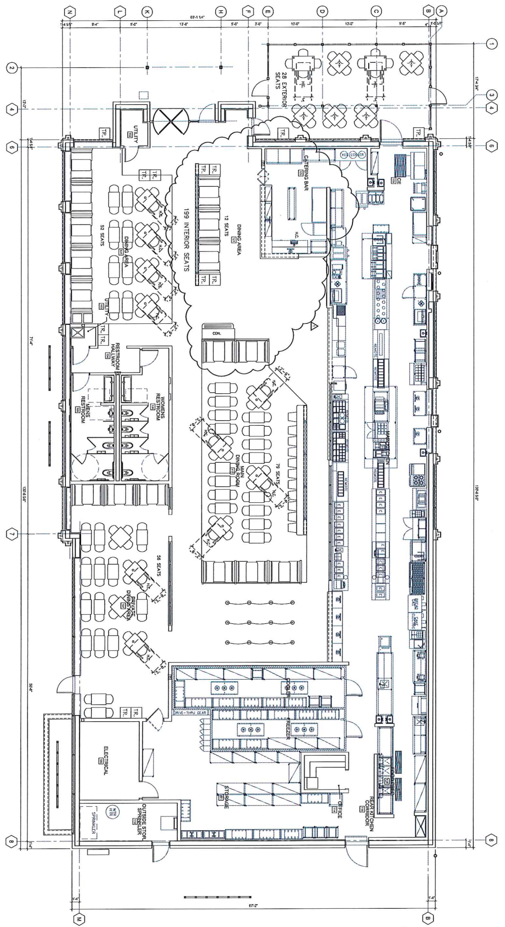
1 FIRST FLOOR SEATING PLAN Scale: 3/16" = 1'-0"
