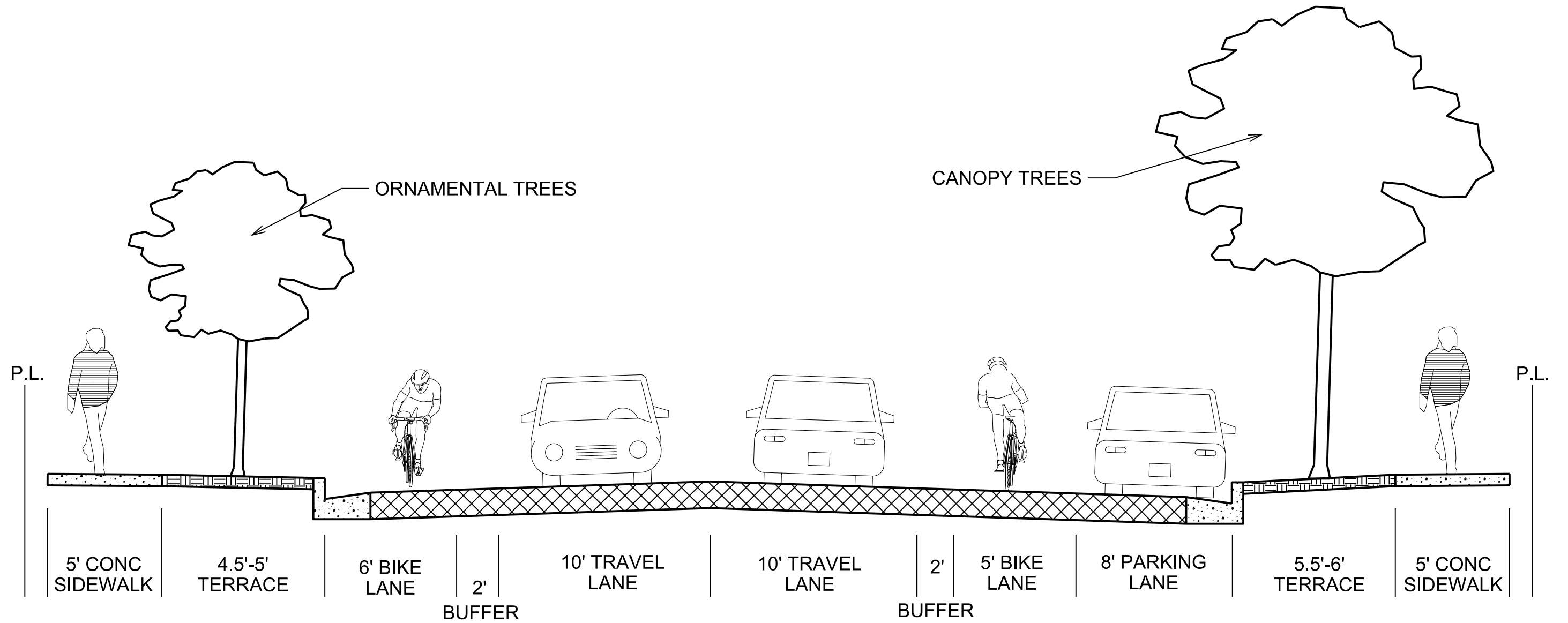
WINNEBAGO STREET - OPTION 2 (LOOKING NORTHEAST)
