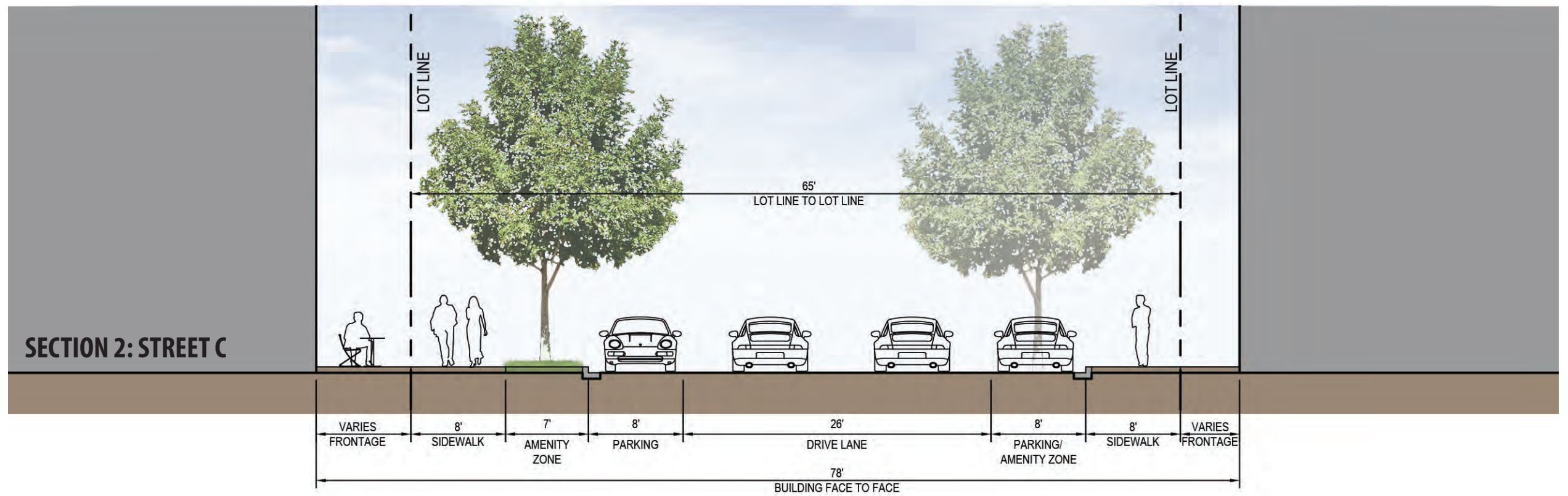
FIGURE 11A - PROPOSED STREET SECTIONS - INTERIOR
