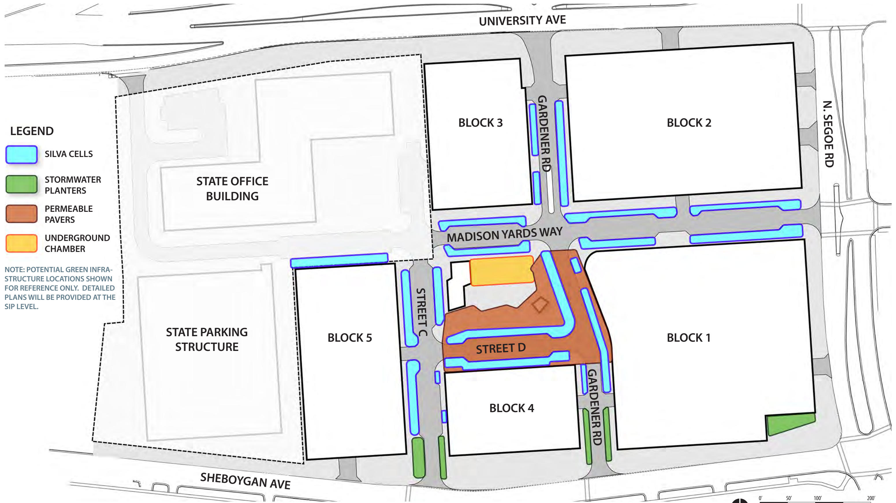
FIGURE 10 - GREEN INFRASTRUCTURE DIAGRAM
