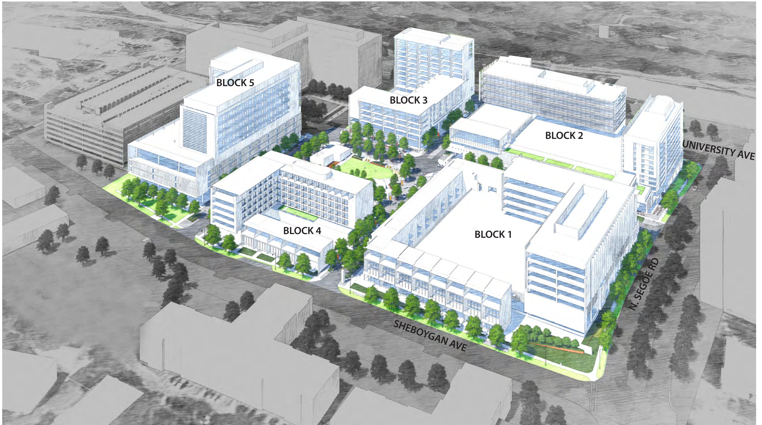
FIGURE 9 - BUILDING MASSING
