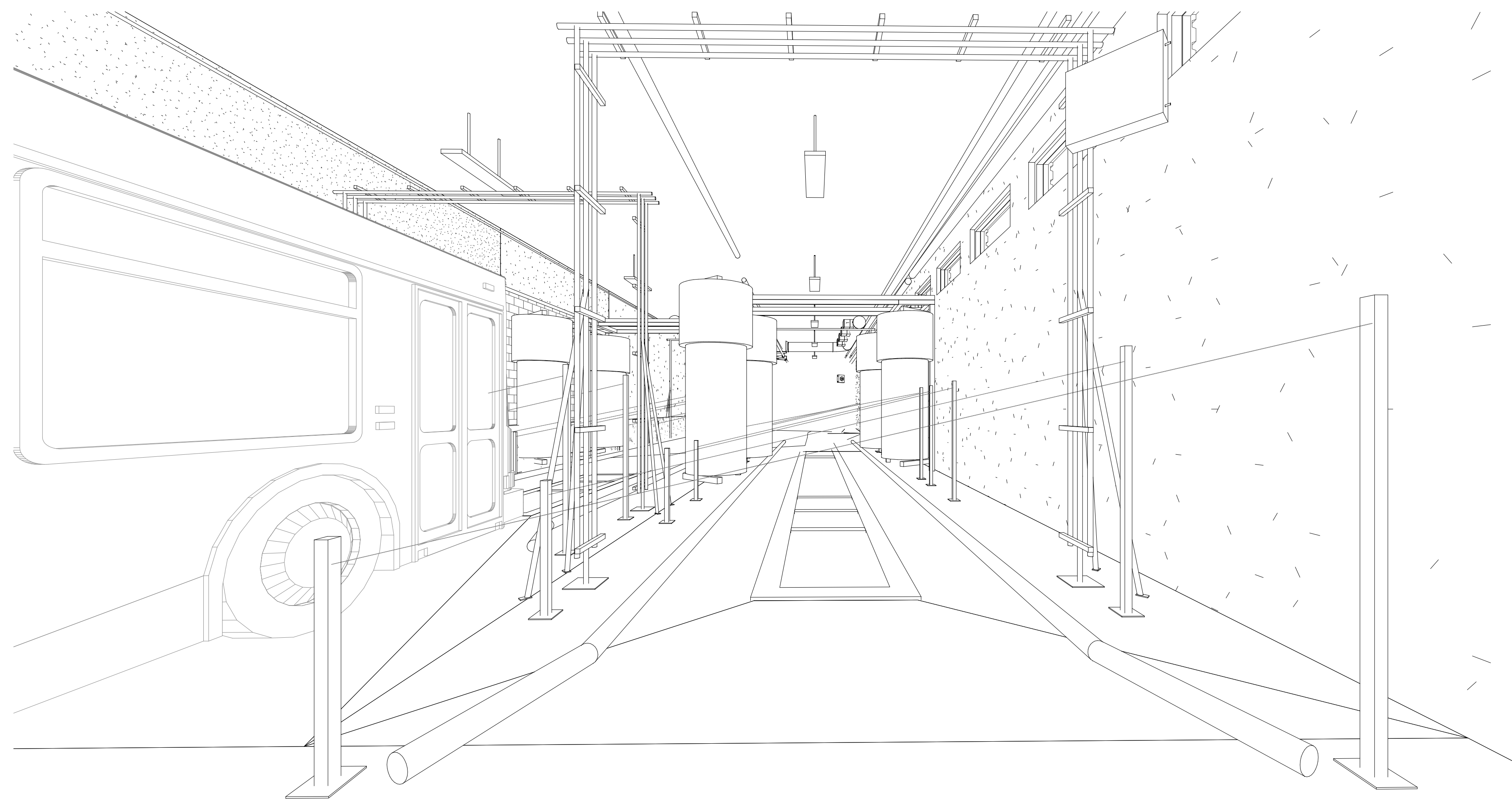
3 INTERIOR 3D PERSPECTIVE - WASH BAY
