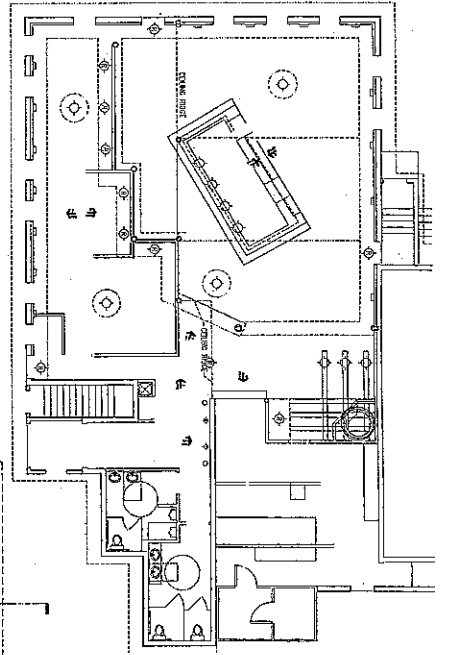
2 REFLECTED CEILING PLAN 1/8" = 1'-0"
