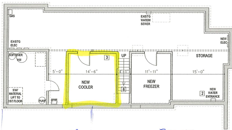
BSMNT FLOOR PLAN
