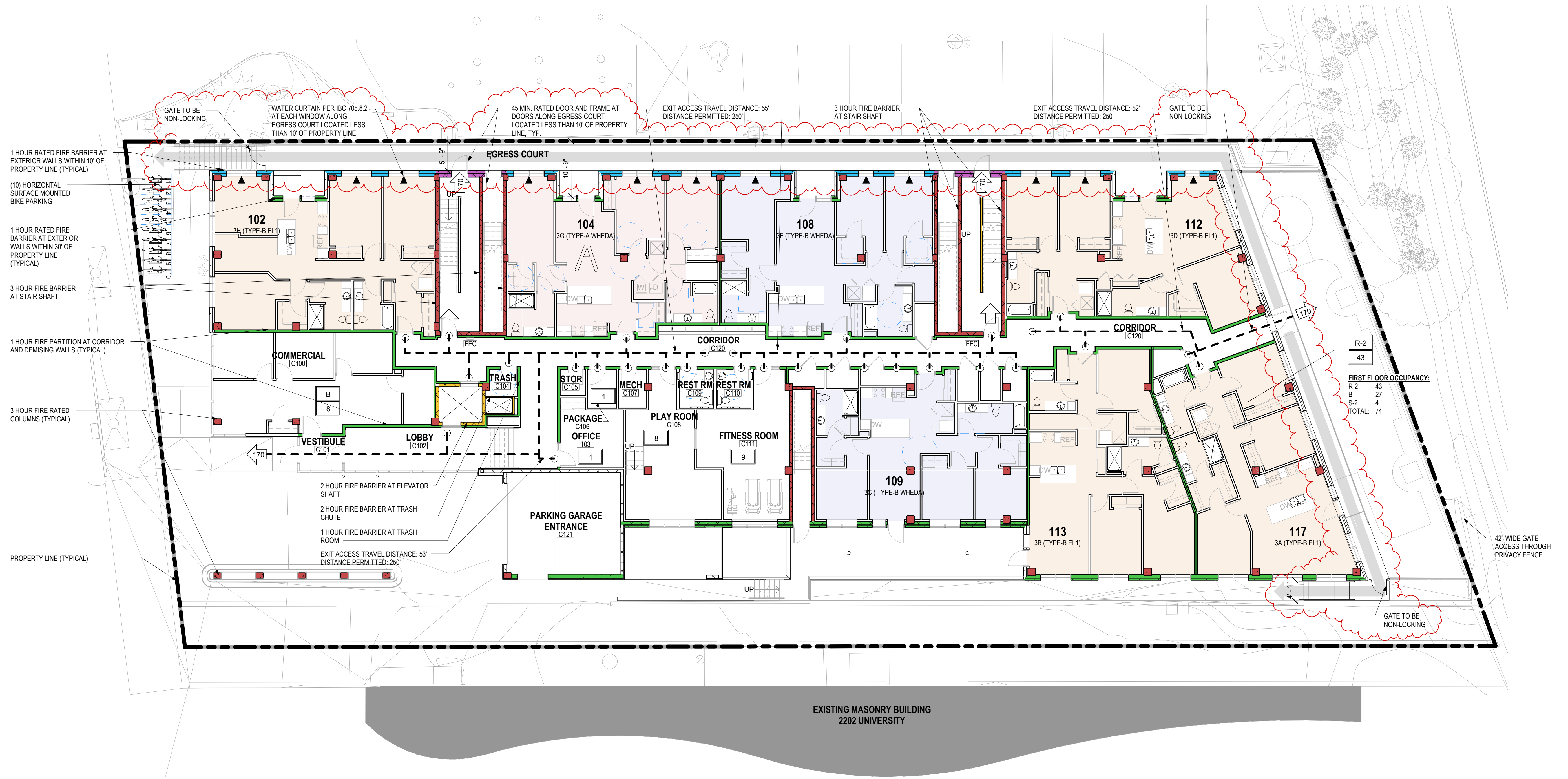
1 FIRST FLOOR CODE COMPLIANCE PLAN 3/32" = 1'-0"
