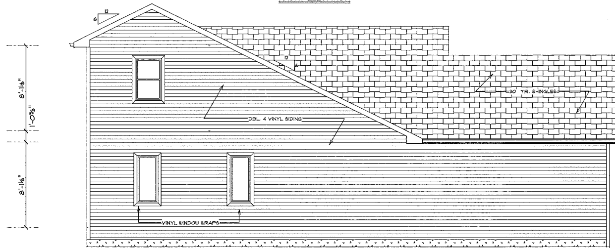
FRONT ELEVATION
