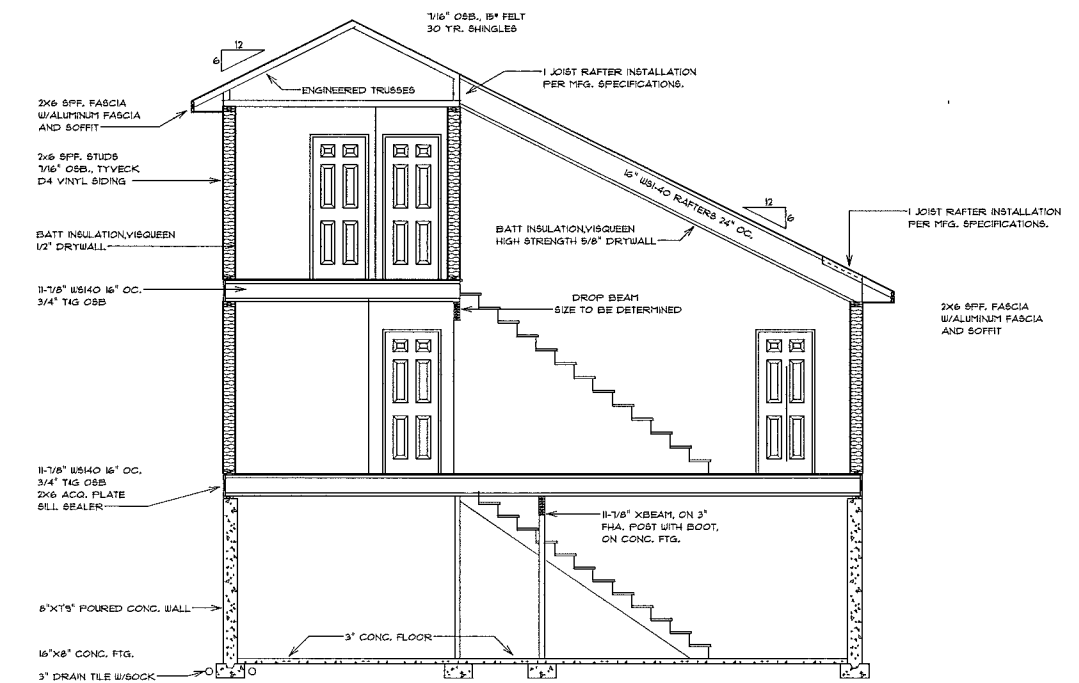
SECTION THROUGH
