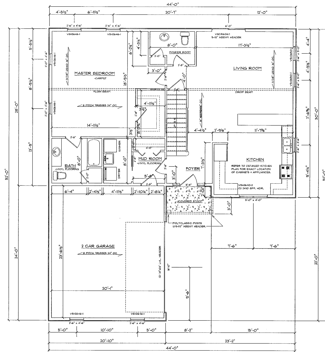
FLOOR PLAN 1277 SQ. FT. 8' CEILINGS VINYL WINDOWS
