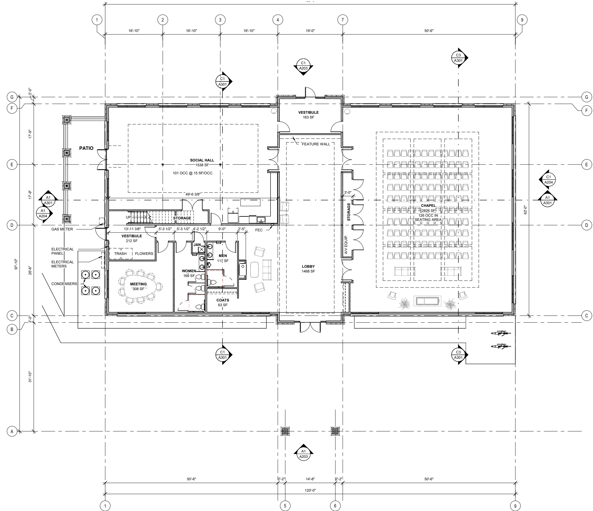
A1 FIRST FLOOR PLAN 1/8" = 1'-0"
