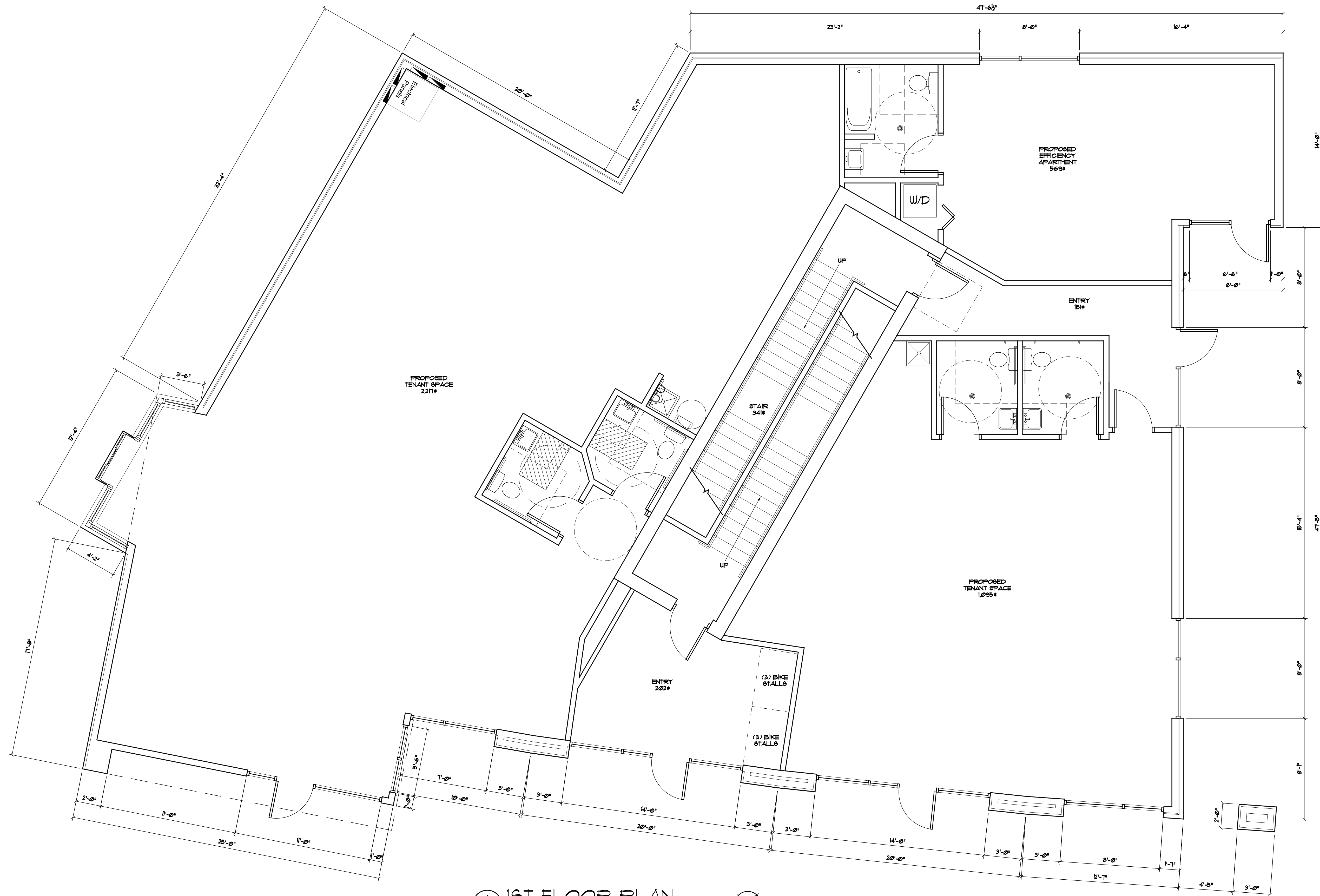
1 1ST FLOOR PLAN A-1.1 SCALE: 1/4" = 1' - 0" NORTH
