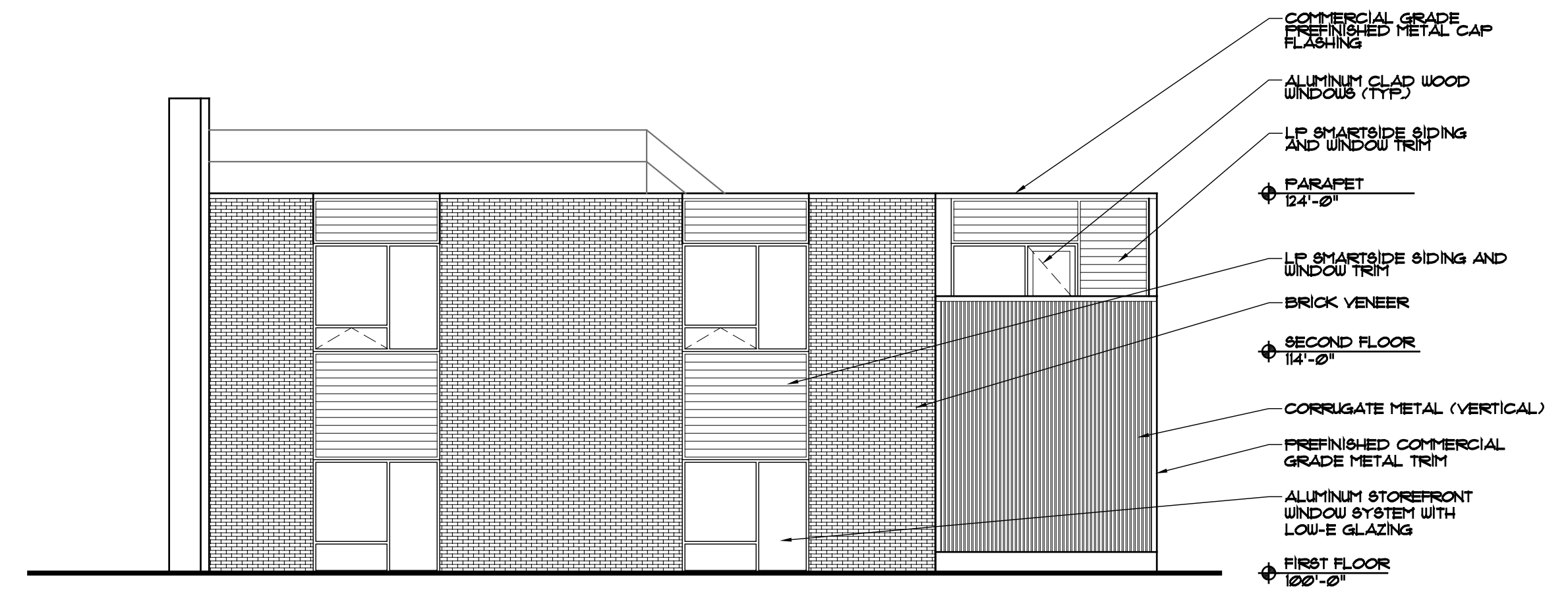
2 PARKING LOT ELEVATION A-2.1 SCALE: 1/8" = 1' - 0"
