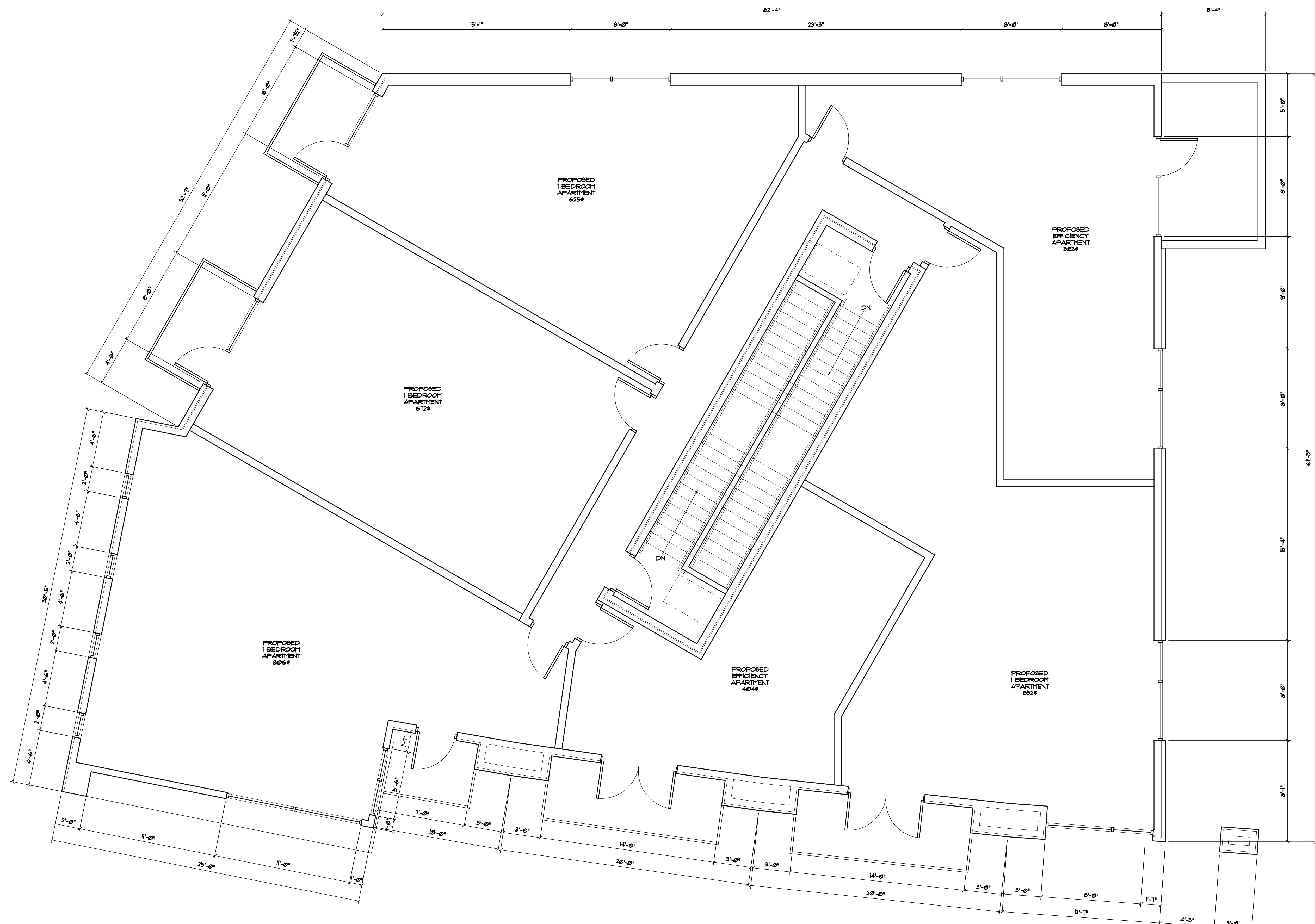
1 2ND FLOOR PLAN A-12 SCALE: 1/4" = 1' - 0" NORTH
