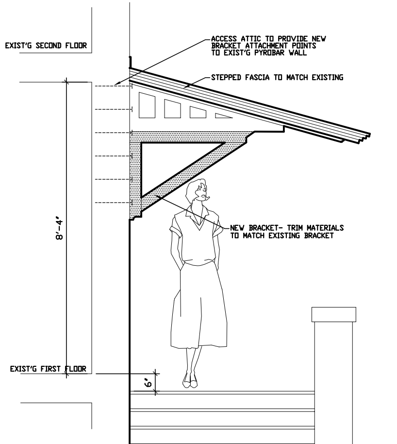
PORCH- SIDE ELEVATION SCALE: 3/8" = 1'-0" PROPOSED
