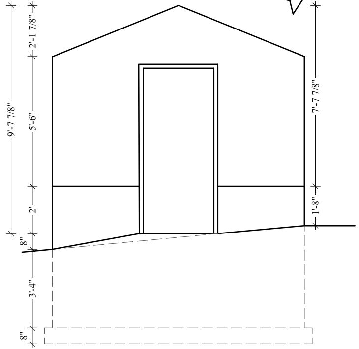
East Elevation
