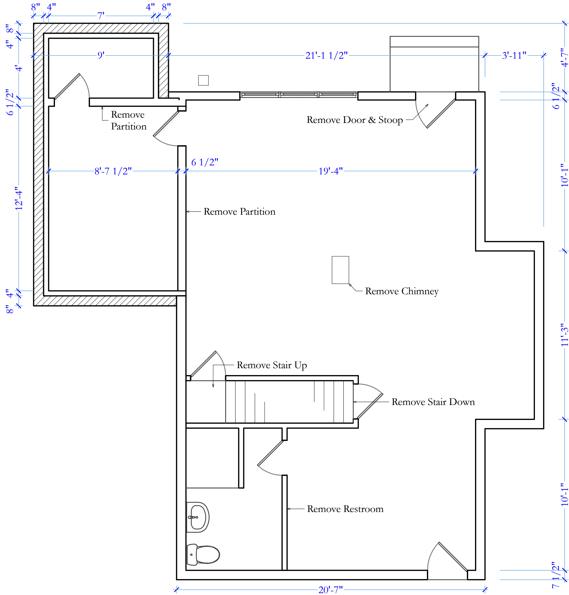
Ground Floor
