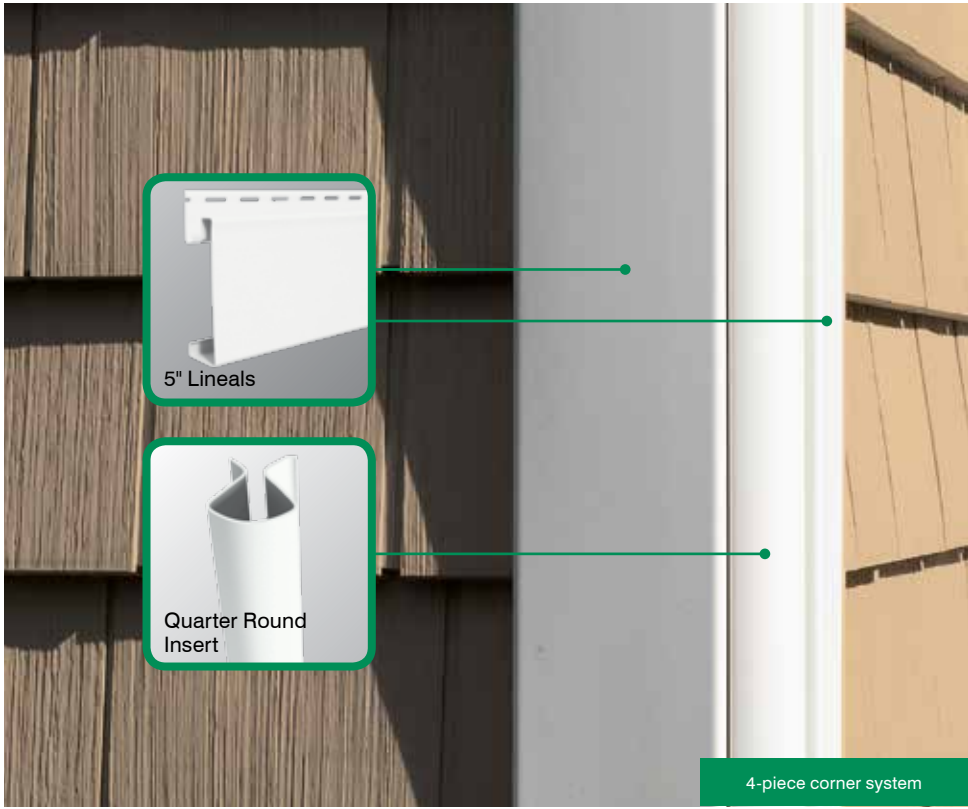
Starter strips are required to build 4 piece corners and federal corners.
