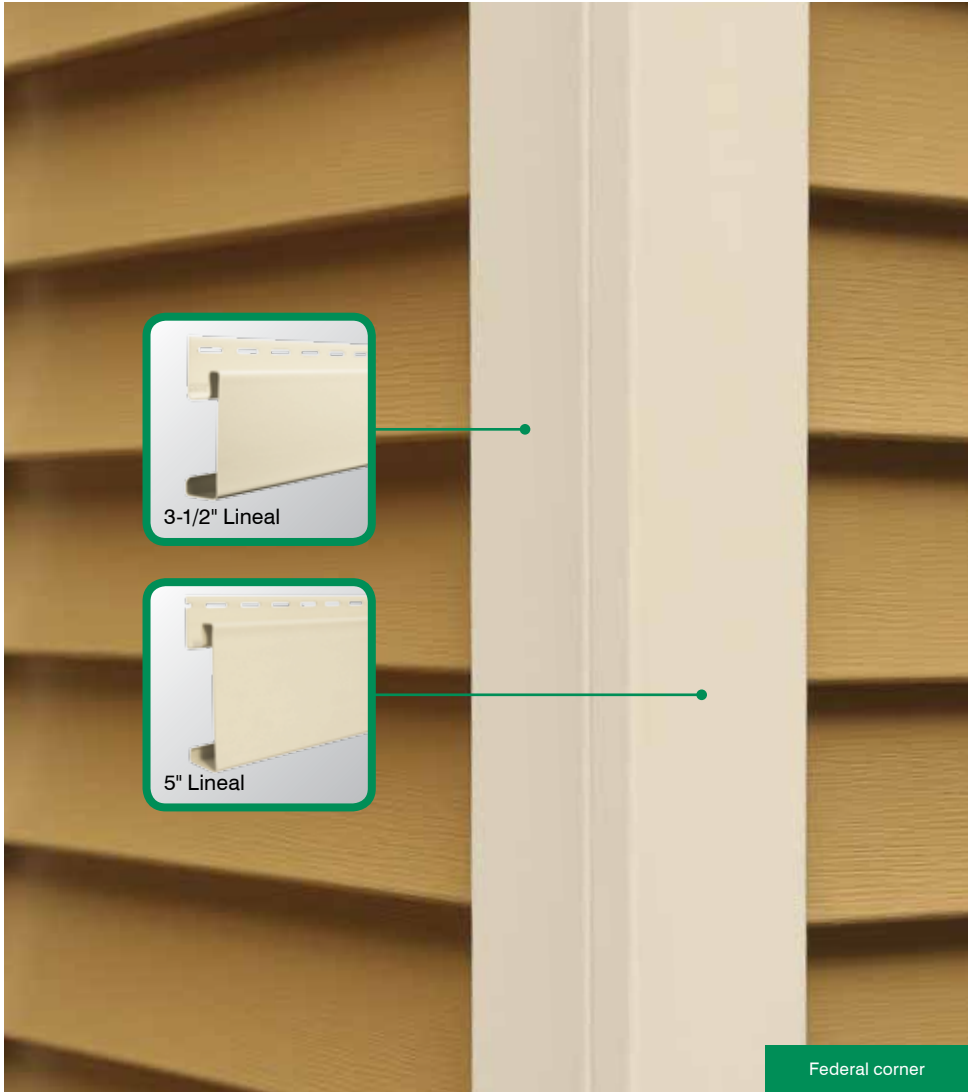
Starter strips are required to build 4 piece corners and federal corners.
