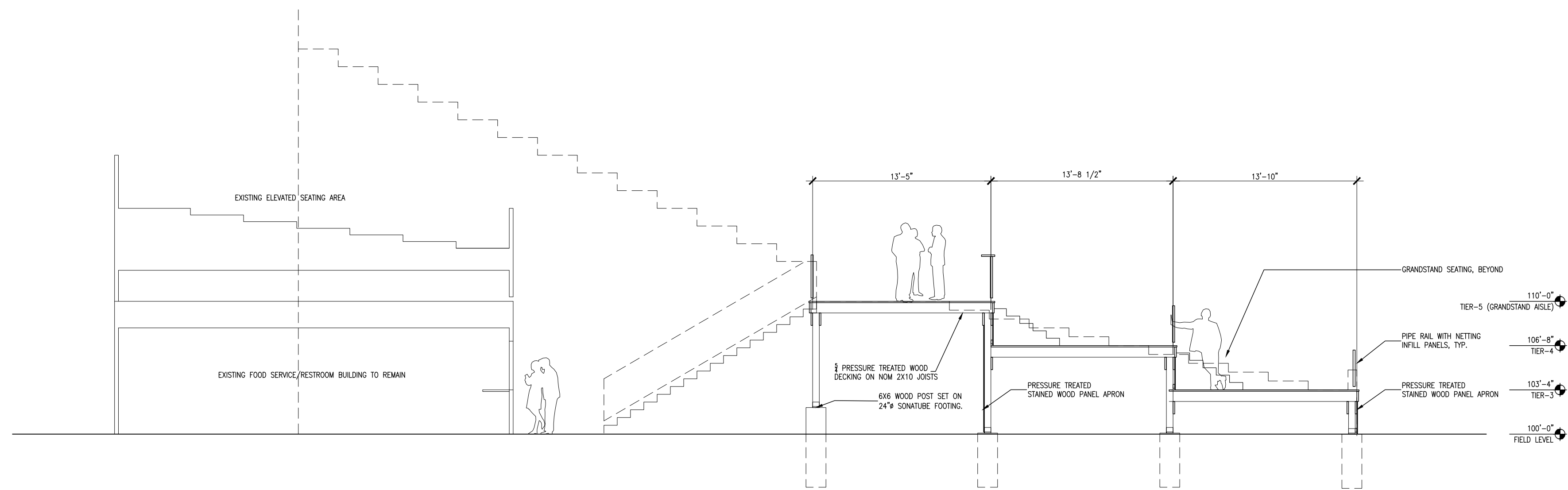
1 DUCK BLIND-WOOD DECK SECTION 1/4"=1'-0"
