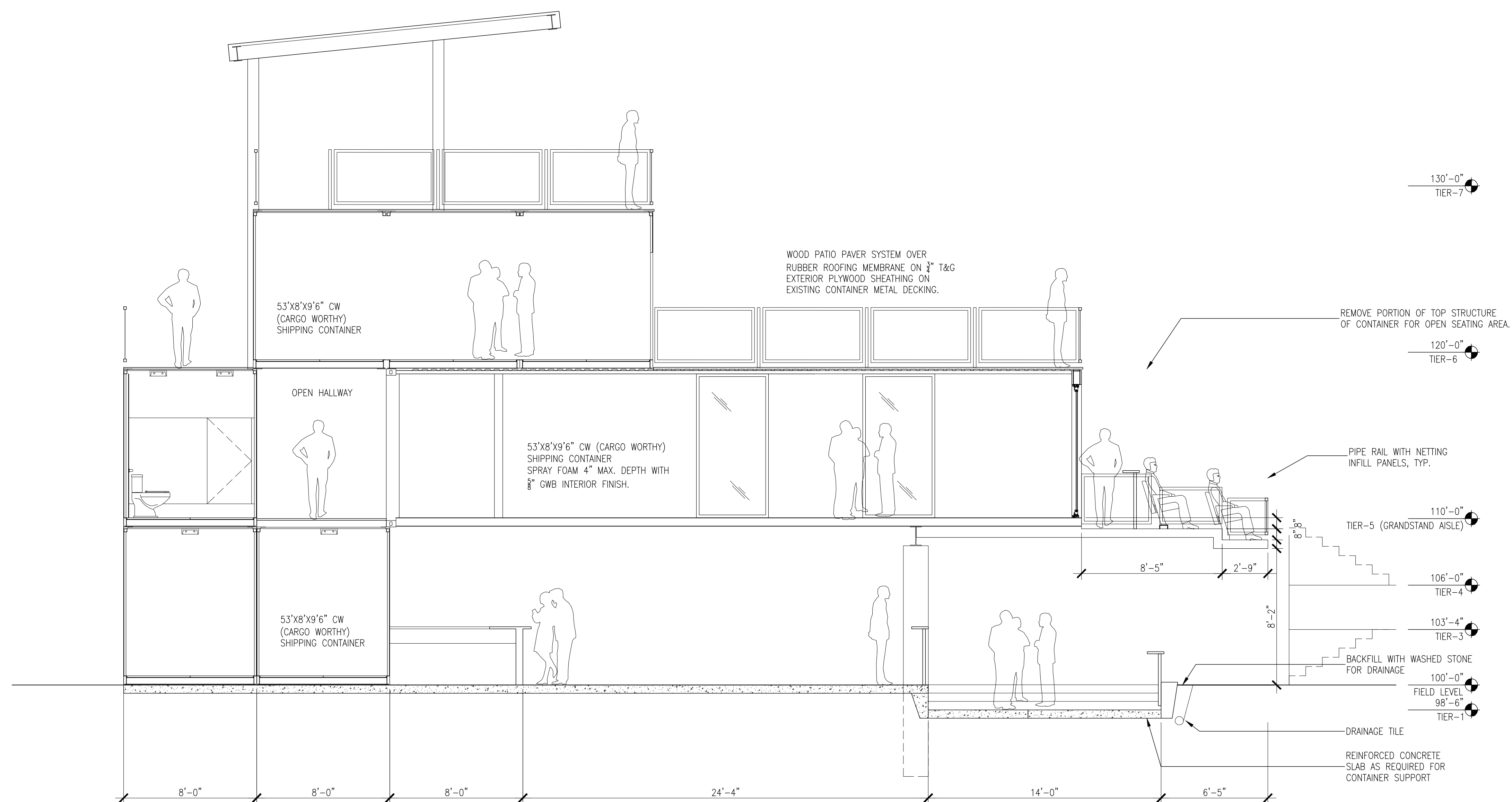
2 DUCK BLIND-SHIPPING CONTAINER SECTION 1/4"=1'-0"
