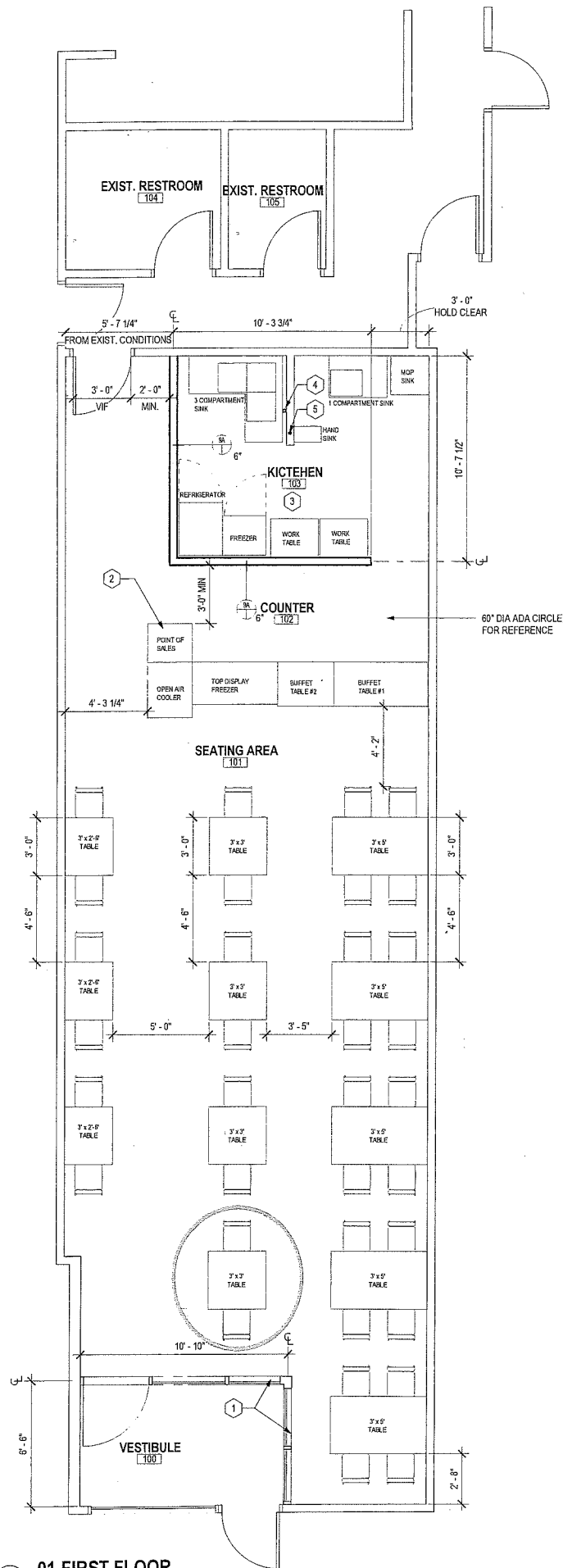
1 01-FIRST FLOOR 1/4" = 1'-0"
