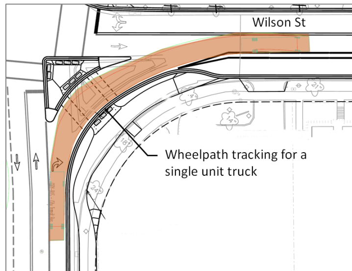
A.2-4 Single Unit Truck Turning Radii
