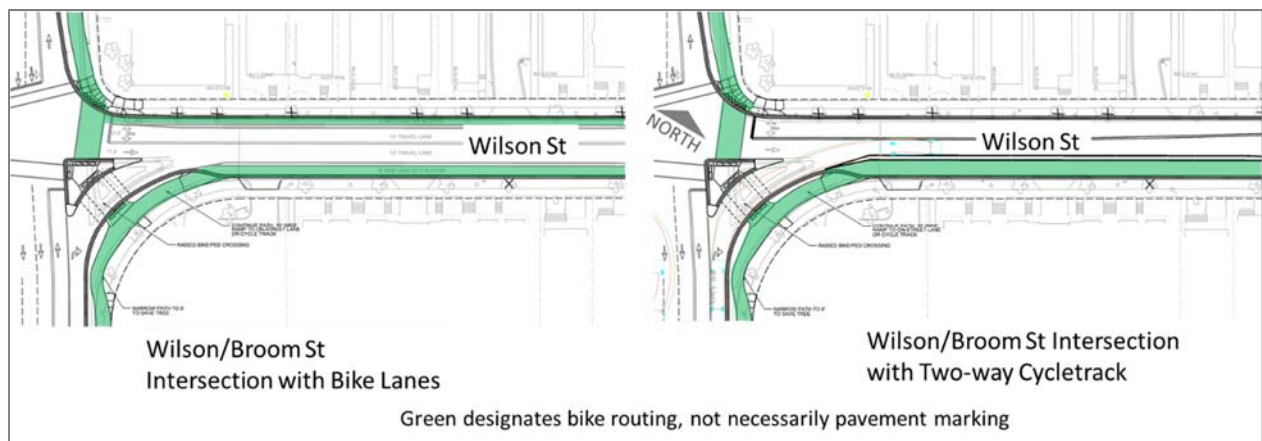
Figure A.5-3 Wilson/Broom Street Intersection with Bike Lanes and Two-way Cycletrack
