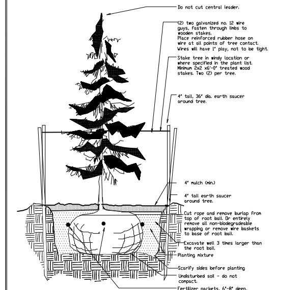
2 EVERGREEN TREE PLANTING Scale - NTS
