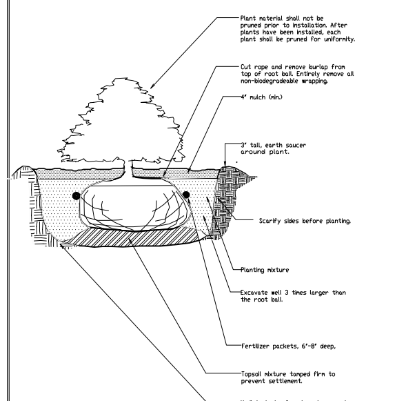
3 SHRUB PLANTING Scale - NTS
