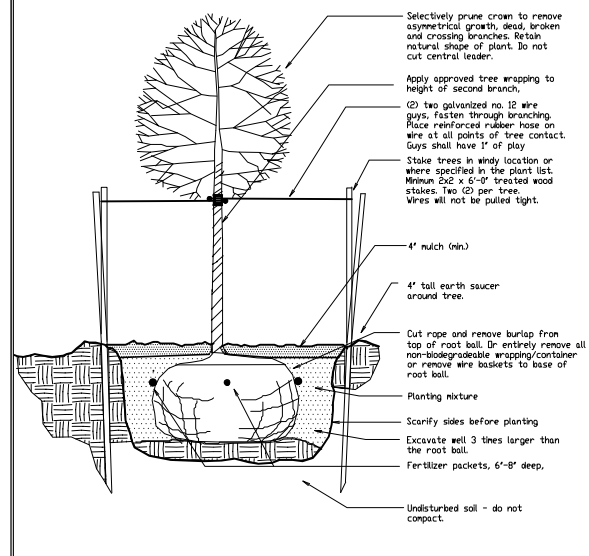
1 SMALL TREE PLANTING (UP TO 2-1/2" CAL.) Scale - NTS
