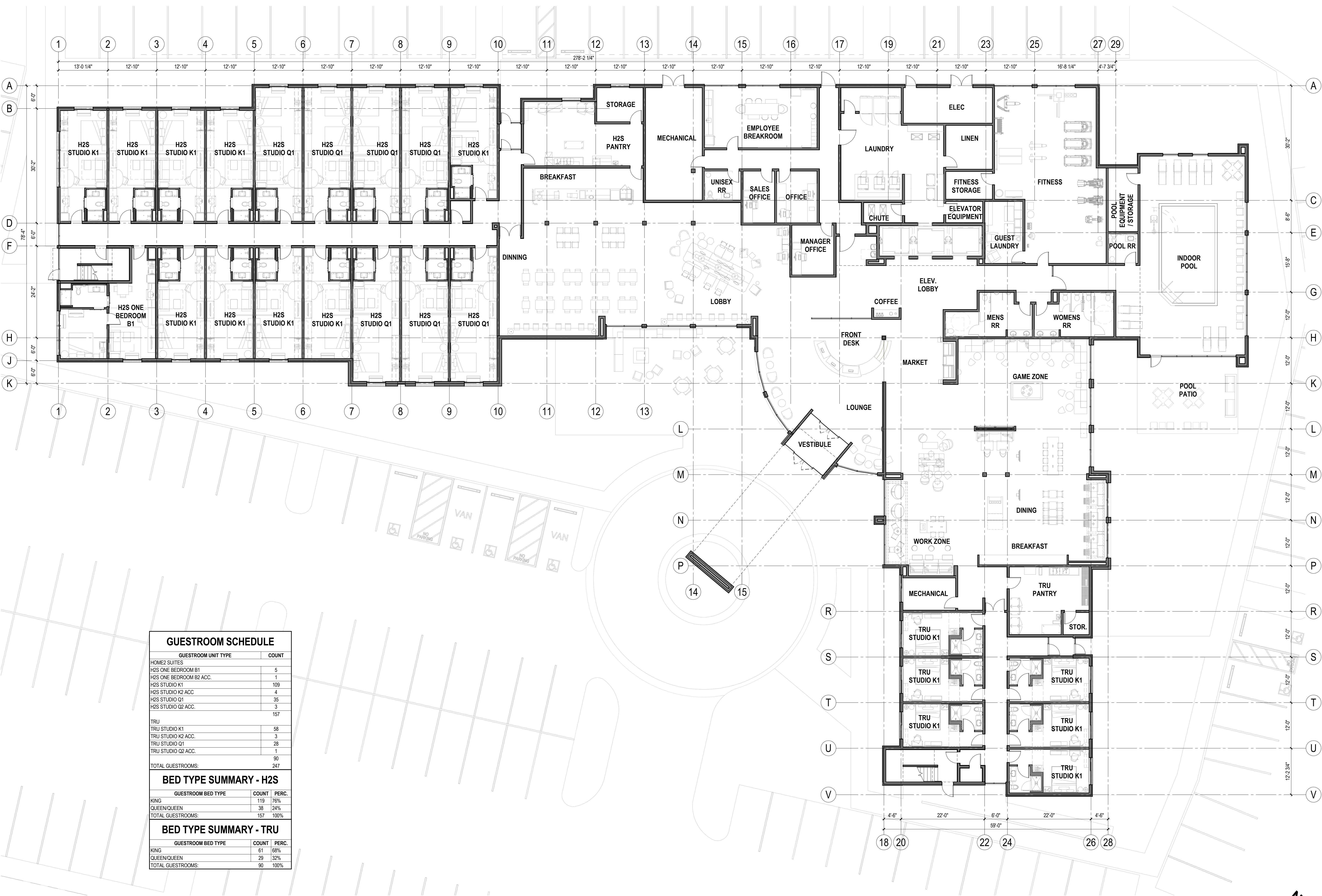
1 FLOOR PLAN - LEVEL 1 3/32" = 1'-0"
