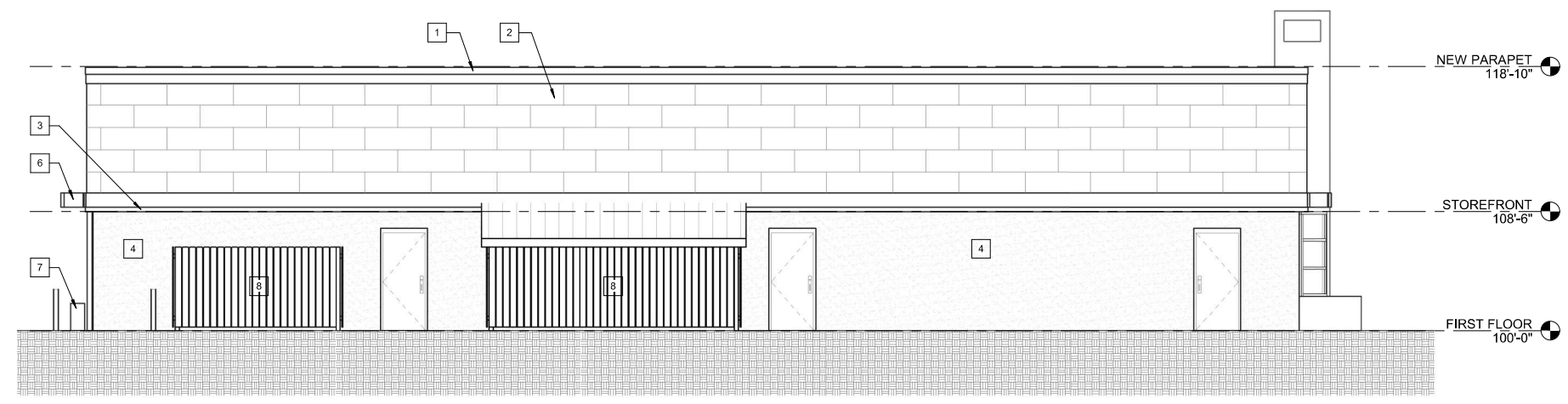
A2 SOUTH ELEVATION 3/16" = 1'-0"
