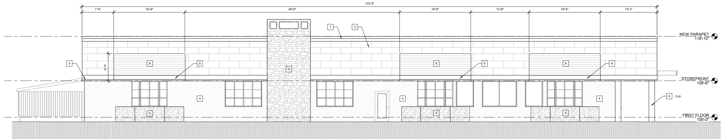
B1 EAST ELEVATION 3/16" = 1'-0"
